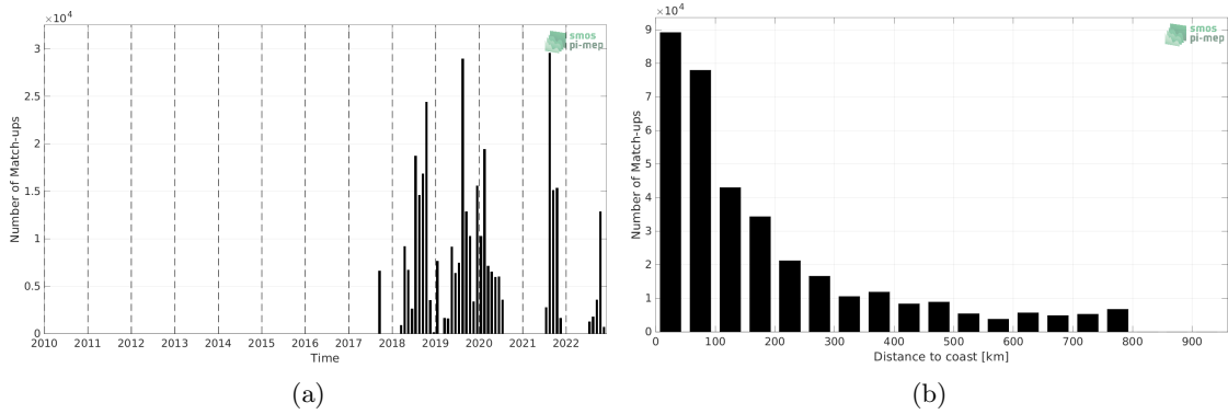
Figure 1: Number of match-ups between Saildrone and SMAP SSS L3 v5 - 8-Day running (RSS) SSS as a function of time (a) and as function of the distance to coast (b) over the SMOS coastal zone (<800km) 60N-60S Pi-MEP region and for the full satellite product period.
