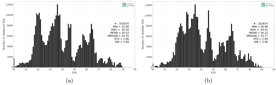
Figure 2: Histograms of SSS from Saildrone (a) and SMAP SSS L3 v5 - 8-Day running (RSS) (b) considering all match-up pairs per bins of 0.1 over the SMOS coastal zone (<800km) 60N-60S Pi-MEP region and for the full satellite product period.
