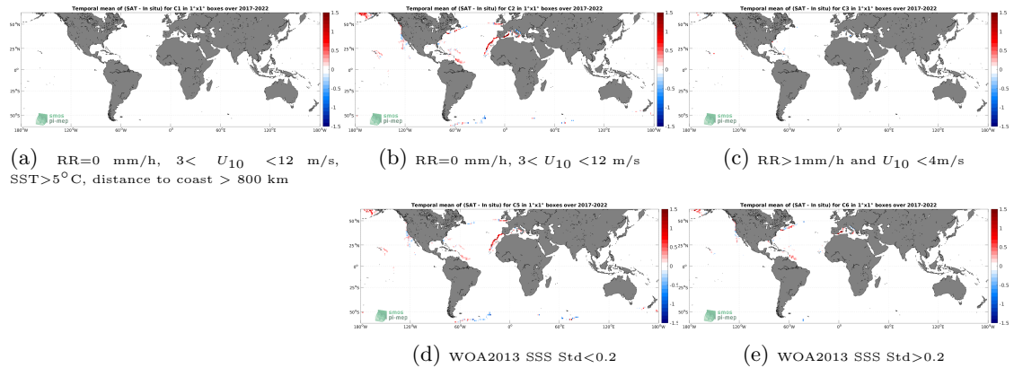
Figure 12: Temporal mean gridded over spatial boxes of size 1^\circ \times 1^\circ of \Delta SSS (SMAP SSS L3 v5 - 8-Day running (RSS) - Saildrone) for 5 different subdatasets corresponding to:RR=0 mm/h, 3 < U_{10} < 12 m/s, SST >5^\circ\text{C} , distance to coast > 800 km (a), RR=0 mm/h, 3 < U_{10} < 12 m/s (b), RR >1 mm/h and U_{10} < 4 m/s (c), WOA2013 SSS Std <0.2 (d), WOA2013 SSS Std >0.2 (e).
