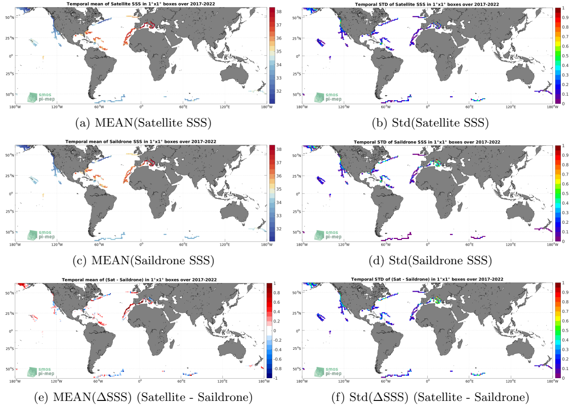
Figure 6: Temporal mean (left) and Std (right) of SSS from SMAP SSS L3 v5 - 8-Day running (RSS) (top), Saildrone (middle), and of \Delta SSS (Satellite - Saildrone). Only match-up pairs are used to generate these maps.
