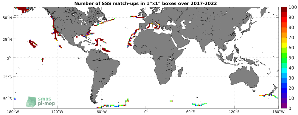
Figure 4: Number of SSS match-ups between Saildrone SSS and the SMAP SSS L3 v5 - 8-Day running (RSS) SSS product for the SMOS coastal zone (<800km) 60N-60S Pi-MEP region over 1^\circ \times 1^\circ boxes and for the full satellite product period.
