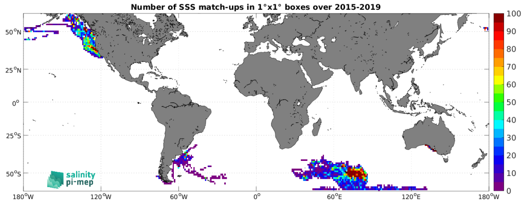
Figure 4: Number of SSS match-ups between Marine mammals SSS and the SMAP SSS L3 v5 - 8-Day running (RSS) SSS product for the SMOS coastal zone (<800km) 60N-60S Pi-MEP region over 1^\circ \times 1^\circ boxes and for the full satellite product period.
