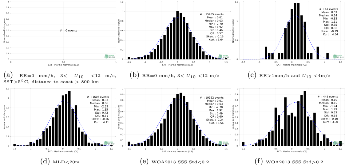
Figure 13: Normalized histogram of \Delta SSS (SMAP SSS L3 v5 - 8-Day running (RSS) - Marine mammals) for 6 different subdatasets corresponding to: RR=0 mm/h, 3 < U_{10} < 12 m/s, SST>5°C, distance to coast > 800 km (a), RR=0 mm/h, 3 < U_{10} < 12 m/s (b), RR>1mm/h and U_{10} < 4 m/s (c), MLD<20m (d), WOA2013 SSS Std<0.2 (e), WOA2013 SSS Std>0.2 (f).
