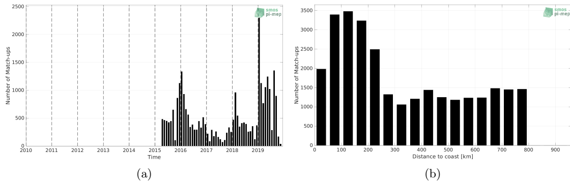
Figure 1: Number of match-ups between Marine mammals and SMAP SSS L3 v5 - 8-Day running (RSS) SSS as a function of time (a) and as function of the distance to coast (b) over the SMOS coastal zone (<800km) 60N-60S Pi-MEP region and for the full satellite product period.
