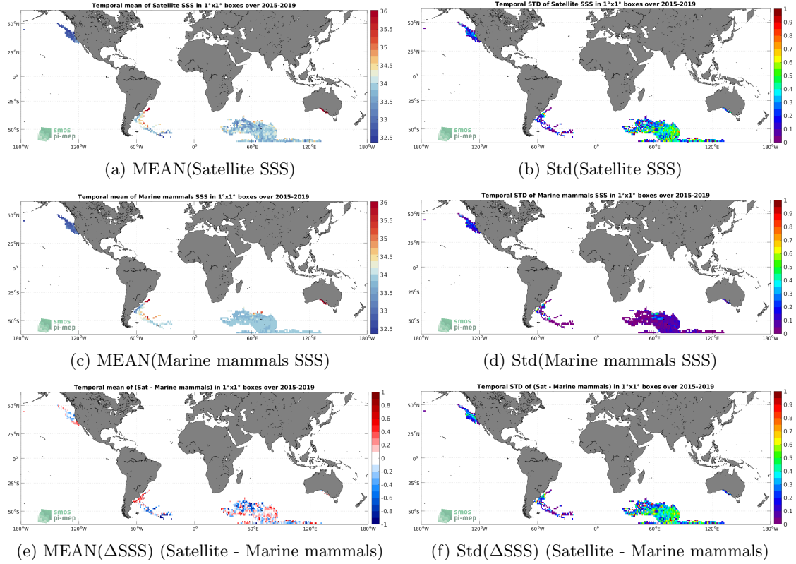
Figure 6: Temporal mean (left) and Std (right) of SSS from SMAP SSS L3 v5 - 8-Day running (RSS) (top), Marine mammals (middle), and of \Delta SSS (Satellite - Marine mammals). Only match-up pairs are used to generate these maps.
