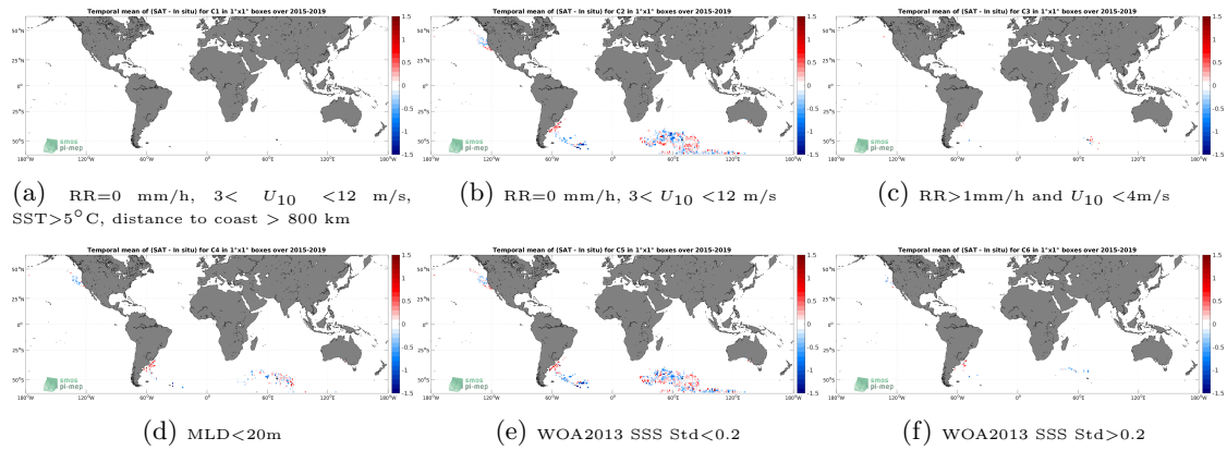
Figure 12: Temporal mean gridded over spatial boxes of size 1^\circ \times 1^\circ of \Delta SSS (SMAP SSS L3 v5 - 8-Day running (RSS) - Marine mammals) for 6 different subdatasets corresponding to:RR=0 mm/h, 3 < U_{10} < 12 m/s, SST >5^\circ C, distance to coast > 800 km (a), RR=0 mm/h, 3 < U_{10} < 12 m/s (b), RR >1 mm/h and U_{10} < 4 m/s (c),MLD <20 m (d),WOA2013 SSS Std <0.2 (e),WOA2013 SSS Std >0.2 (f).
