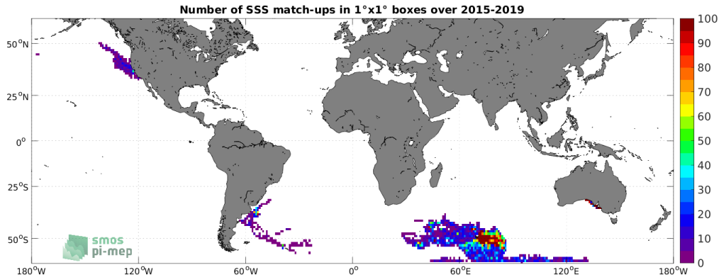
Figure 4: Number of SSS match-ups between Marine mammals SSS and the SMAP SSS L3 v5 - 8-Day running (RSS) SSS product for the SMOS coastal zone (<800km) 60N-60S Pi-MEP region over 1^{\circ} \times 1^{\circ} boxes and for the full satellite product period.
