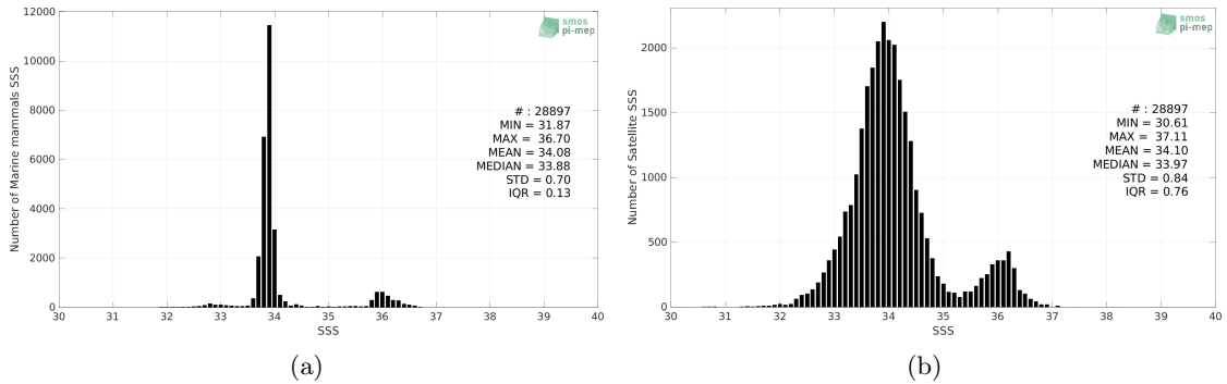
Figure 2: Histograms of SSS from Marine mammals (a) and SMAP SSS L3 v5 - 8-Day running (RSS) (b) considering all match-up pairs per bins of 0.1 over the SMOS coastal zone (<800km) 60N-60S Pi-MEP region and for the full satellite product period.
