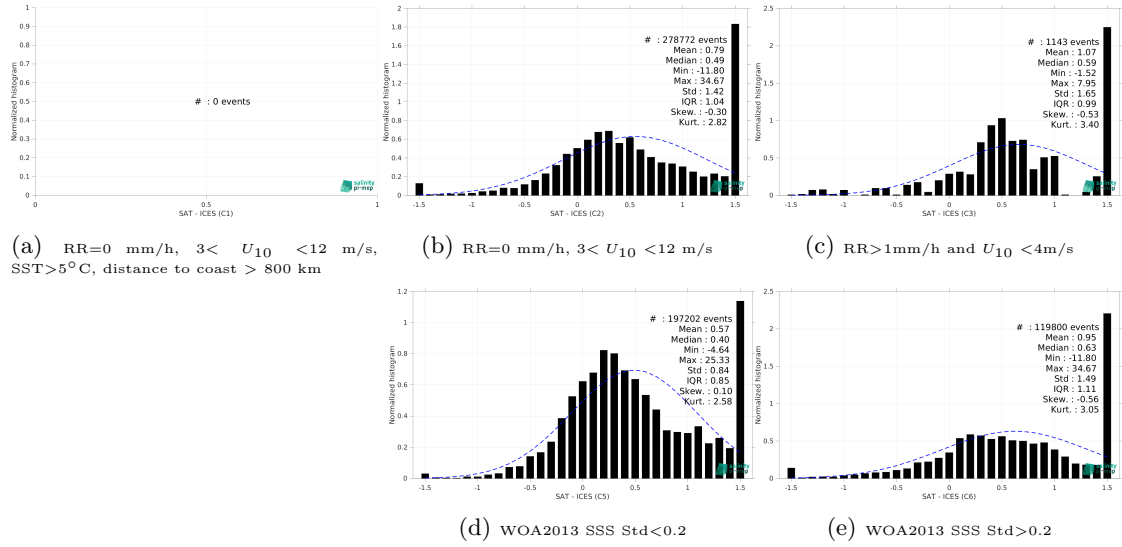
Figure 13: Normalized histogram of \Delta SSS (SMAP SSS L3 v5 - 8-Day running (RSS) - ICES) for 5 different subdatasets corresponding to: RR=0 mm/h, 3 < U_{10} < 12 m/s, SST>5°C, distance to coast > 800 km (a), RR=0 mm/h, 3 < U_{10} < 12 m/s (b), RR>1mm/h and U_{10} < 4 m/s (c), WOA2013 SSS Std<0.2 (d), WOA2013 SSS Std>0.2 (e).
