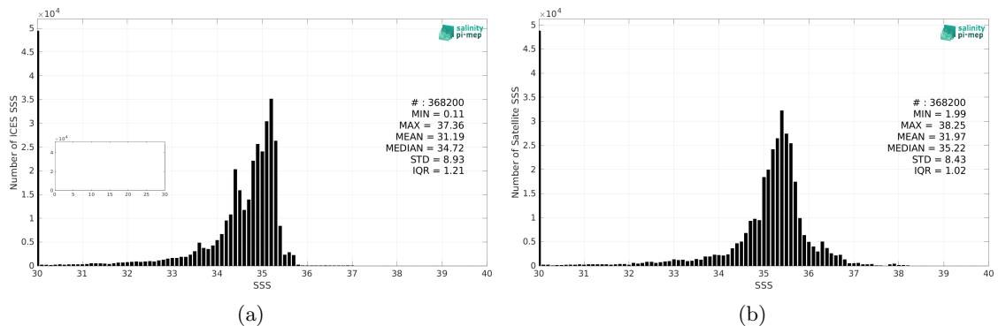
Figure 2: Histograms of SSS from ICES (a) and SMAP SSS L3 v5 - 8-Day running (RSS) (b) considering all match-up pairs per bins of 0.1 over the SMOS coastal zone (<800km) 60N-60S Pi-MEP region and for the full satellite product period.
