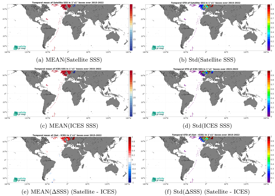
Figure 6: Temporal mean (left) and Std (right) of SSS from SMAP SSS L3 v5 - 8-Day running (RSS) (top), ICES (middle), and of \Delta SSS (Satellite - ICES). Only match-up pairs are used to generate these maps.
