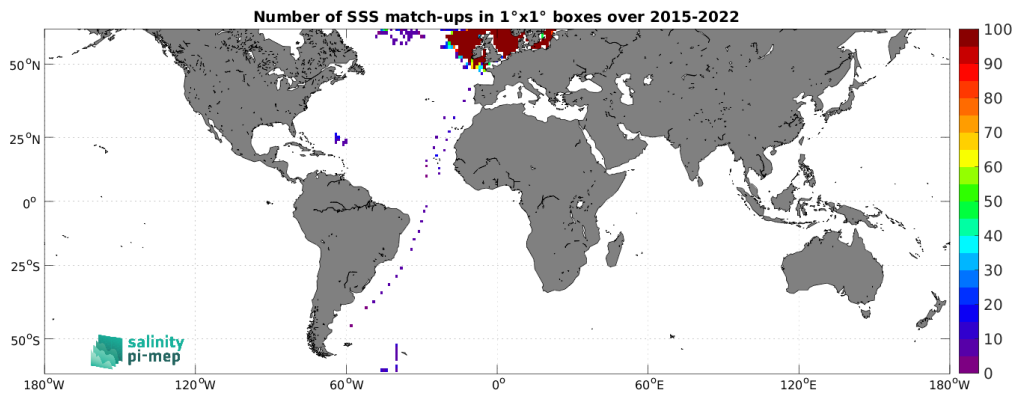
Figure 4: Number of SSS match-ups between ICES SSS and the SMAP SSS L3 v5 - 8-Day running (RSS) SSS product for the SMOS coastal zone (<800km) 60N-60S Pi-MEP region over 1^\circ \times 1^\circ boxes and for the full satellite product period.
