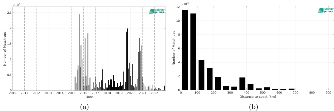
Figure 1: Number of match-ups between ICES and SMAP SSS L3 v5 - 8-Day running (RSS) SSS as a function of time (a) and as function of the distance to coast (b) over the SMOS coastal zone (<800km) 60N-60S Pi-MEP region and for the full satellite product period.
