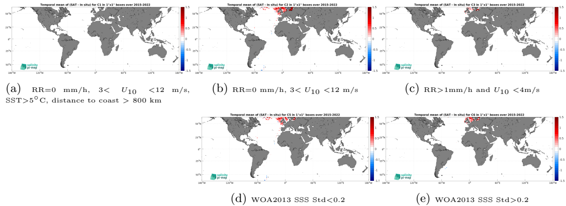
Figure 12: Temporal mean gridded over spatial boxes of size 1^\circ \times 1^\circ of \Delta\text{SSS} (SMAP SSS L3 v5 - 8-Day running (RSS) - ICES) for 5 different subdatasets corresponding to:RR=0 mm/h, 3 < U_{10} < 12 m/s, SST >5^\circ\text{C} , distance to coast > 800 km (a), RR=0 mm/h, 3 < U_{10} < 12 m/s (b), RR >1 mm/h and U_{10} < 4 m/s (c), WOA2013 SSS Std <0.2 (d), WOA2013 SSS Std >0.2 (e).
