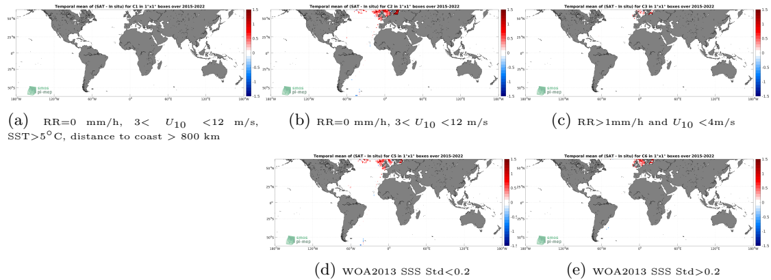
Figure 12: Temporal mean gridded over spatial boxes of size 1^\circ \times 1^\circ of \Delta SSS (SMAP SSS L3 v5 - 8-Day running (RSS) - ICES) for 5 different subdatasets corresponding to:RR=0 mm/h, 3 < U_{10} < 12 m/s, SST >5^\circ\text{C} , distance to coast > 800 km (a), RR=0 mm/h, 3 < U_{10} < 12 m/s (b), RR >1 mm/h and U_{10} < 4 m/s (c), WOA2013 SSS Std <0.2 (d), WOA2013 SSS Std >0.2 (e).
