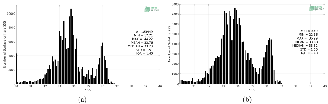
Figure 2: Histograms of SSS from Surface drifters (a) and SMAP SSS L3 v5 - 8-Day running (RSS) (b) considering all match-up pairs per bins of 0.1 over the SMOS coastal zone (<800km) 60N-60S Pi-MEP region and for the full satellite product period.
