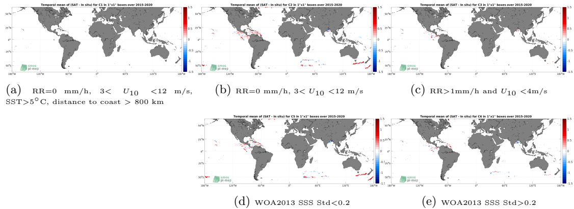
Figure 11: Temporal mean gridded over spatial boxes of size 1^\circ \times 1^\circ of \Delta SSS (SMAP SSS L3 v5 - 8-Day running (RSS) - Surface drifters) for 5 different subdatasets corresponding to:RR=0 mm/h, 3 < U_{10} < 12 m/s, SST >5^\circ C, distance to coast > 800 km (a), RR=0 mm/h, 3 < U_{10} < 12 m/s (b), RR >1 mm/h and U_{10} < 4 m/s (c), WOA2013 SSS Std <0.2 (d), WOA2013 SSS Std >0.2 (e).
