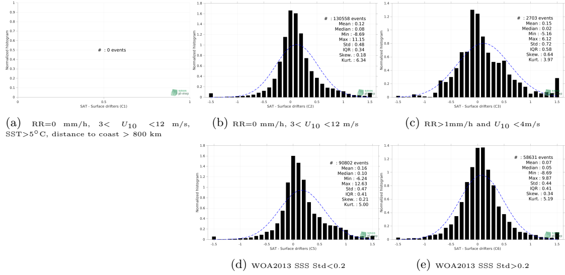
Figure 12: Normalized histogram of \Delta SSS (SMAP SSS L3 v5 - 8-Day running (RSS) - Surface drifters) for 5 different subdatasets corresponding to: RR=0 mm/h, 3 < U_{10} < 12 m/s, SST>5°C, distance to coast > 800 km (a), RR=0 mm/h, 3 < U_{10} < 12 m/s (b), RR>1mm/h and U_{10} < 4 m/s (c), WOA2013 SSS Std<0.2 (d), WOA2013 SSS Std>0.2 (e).
