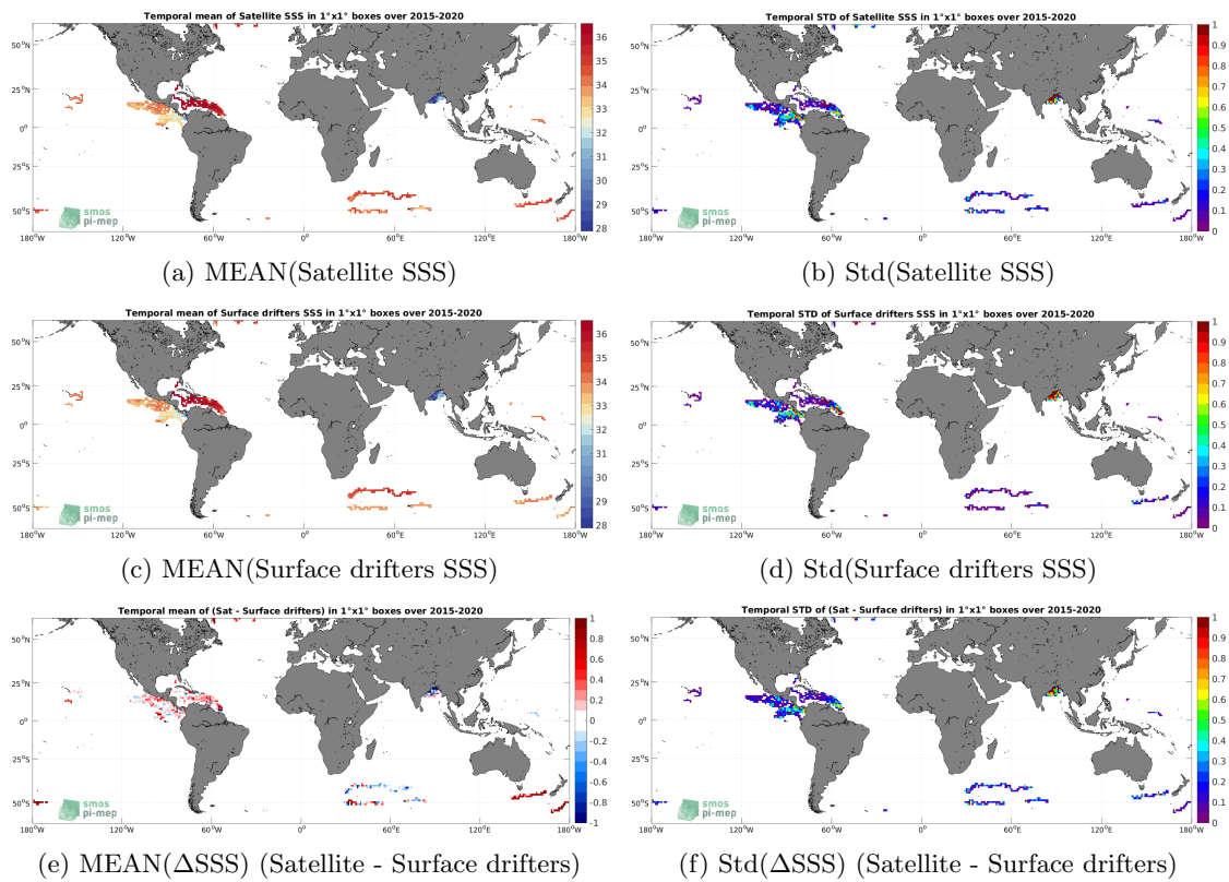
Figure 5: Temporal mean (left) and Std (right) of SSS from SMAP SSS L3 v5 - 8-Day running (RSS) (top), Surface drifters (middle), and of \Delta SSS (Satellite - Surface drifters). Only match-up pairs are used to generate these maps.
