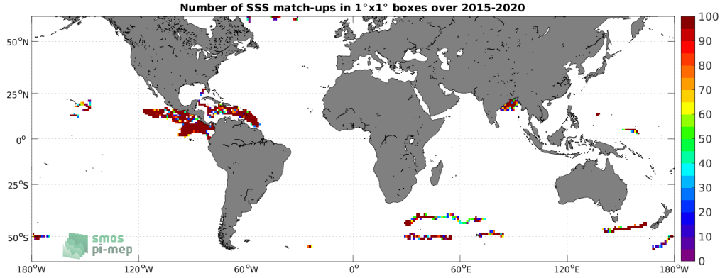
Figure 3: Number of SSS match-ups between Surface drifters SSS and the SMAP SSS L3 v5 - 8-Day running (RSS) SSS product for the SMOS coastal zone (<800km) 60N-60S Pi-MEP region over 1^\circ \times 1^\circ boxes and for the full satellite product period.
