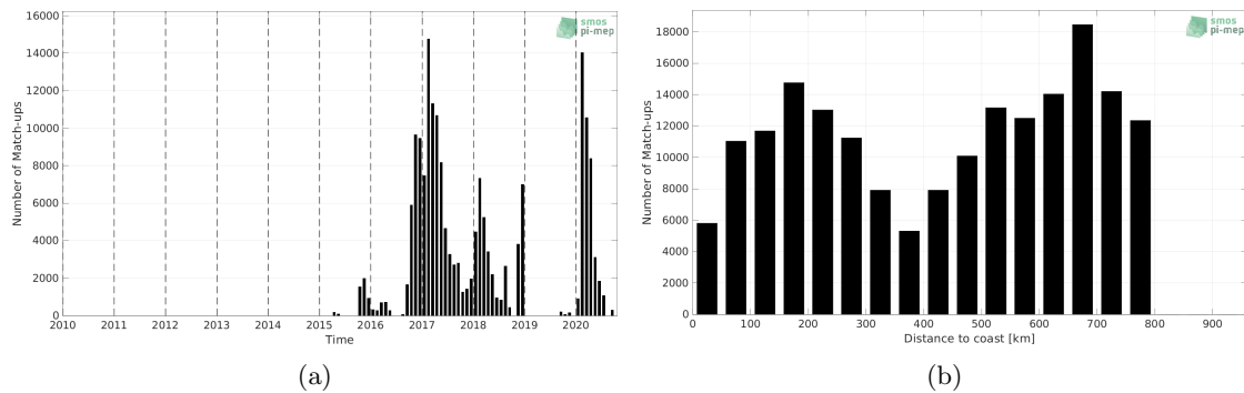
Figure 1: Number of match-ups between Surface drifters and SMAP SSS L3 v5 - 8-Day running (RSS) SSS as a function of time (a) and as function of the distance to coast (b) over the SMOS coastal zone (<800km) 60N-60S Pi-MEP region and for the full satellite product period.
