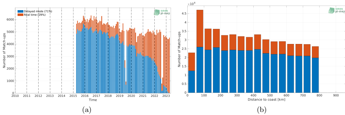
Figure 1: Number of match-ups between Argo and SMAP SSS L3 v5 - 8-Day running (RSS) SSS as a function of time (a) and as function of the distance to coast (b) over the SMOS coastal zone (<800km) 60N-60S Pi-MEP region and for the full satellite product period.
