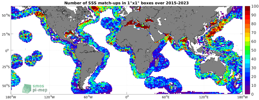
Figure 4: Number of SSS match-ups between Argo SSS and the SMAP SSS L3 v5 - 8-Day running (RSS) SSS product for the SMOS coastal zone ( <800\text{km} ) 60N-60S Pi-MEP region over 1^\circ \times 1^\circ boxes and for the full satellite product period.
