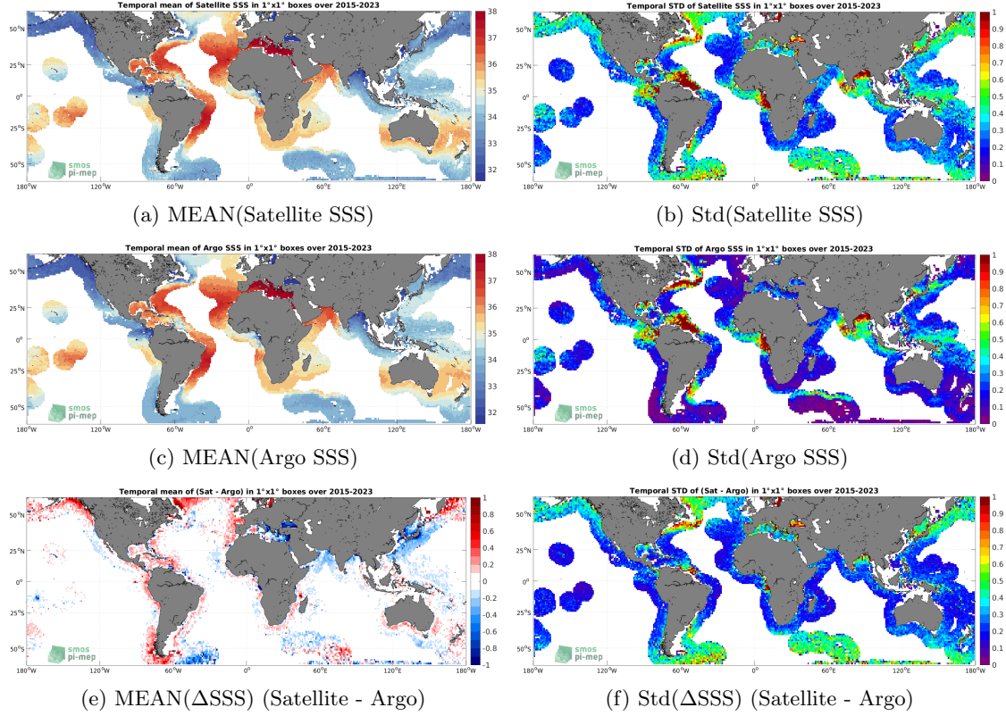
Figure 6: Temporal mean (left) and Std (right) of SSS from SMAP SSS L3 v5 - 8-Day running (RSS) (top), Argo (middle), and of \Delta SSS (Satellite - Argo). Only match-up pairs are used to generate these maps.
