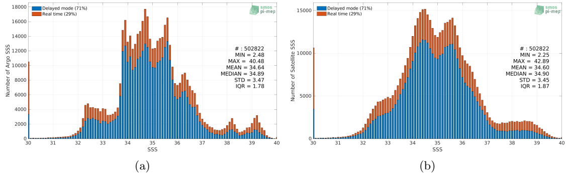
Figure 2: Histograms of SSS from Argo (a) and SMAP SSS L3 v5 - 8-Day running (RSS) (b) considering all match-up pairs per bins of 0.1 over the SMOS coastal zone (<800km) 60N-60S Pi-MEP region and for the full satellite product period.
