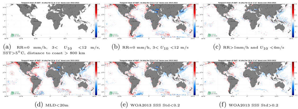
Figure 12: Temporal mean gridded over spatial boxes of size 1^\circ \times 1^\circ of \Delta SSS (SMAP SSS L3 v5 - 8-Day running (RSS) - Argo) for 6 different subdatasets corresponding to:RR=0 mm/h, 3 < U_{10} < 12 m/s, SST >5^\circ C, distance to coast > 800 km (a), RR=0 mm/h, 3 < U_{10} < 12 m/s (b), RR >1 mm/h and U_{10} < 4 m/s (c),MLD <20 m (d),WOA2013 SSS Std <0.2 (e),WOA2013 SSS Std >0.2 (f).
