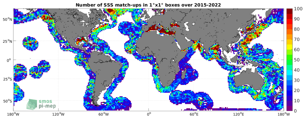
Figure 4: Number of SSS match-ups between Argo SSS and the SMAP SSS L3 v5 - 8-Day running (RSS) SSS product for the SMOS coastal zone (<800km) 60N-60S Pi-MEP region over 1^\circ \times 1^\circ boxes and for the full satellite product period.
