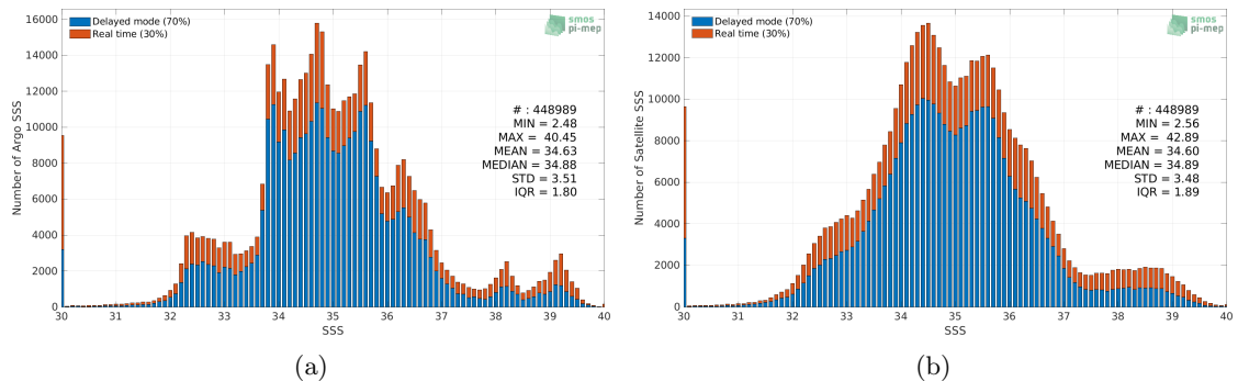
Figure 2: Histograms of SSS from Argo (a) and SMAP SSS L3 v5 - 8-Day running (RSS) (b) considering all match-up pairs per bins of 0.1 over the SMOS coastal zone (<800km) 60N-60S Pi-MEP region and for the full satellite product period.
