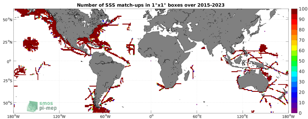
Figure 4: Number of SSS match-ups between TSG (SAMOS) SSS and the SMAP SSS L3 v5 - Monthly (RSS) SSS product for the SMOS coastal zone (<800km) 60N-60S Pi-MEP region over 1°×1° boxes and for the full satellite product period.
