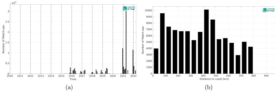
Figure 1: Number of match-ups between TSG (Polarstern) and SMAP SSS L3 v5 - Monthly (RSS) SSS as a function of time (a) and as function of the distance to coast (b) over the SMOS coastal zone (<800km) 60N-60S Pi-MEP region and for the full satellite product period.
