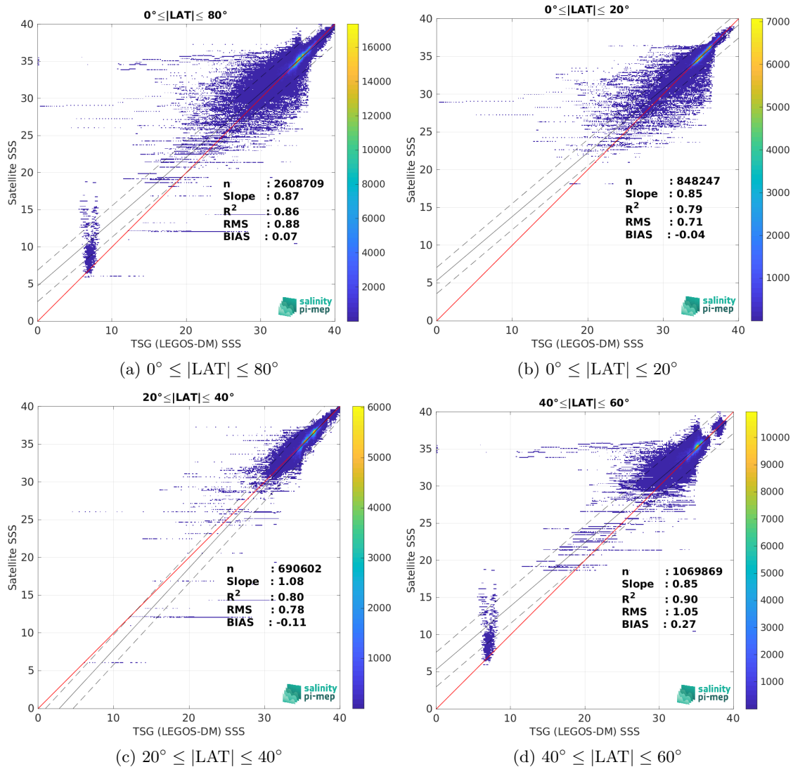
Figure 9: Contour maps of the concentration of SMAP SSS L3 v5 - Monthly (RSS) SSS (y-axis) versus TSG (LEGOS-DM) SSS (x-axis) at match-up pairs for different latitude bands. For each plot, the red line shows x=y . The black thin and dashed lines indicate a linear fit through the data cloud and the \pm 95\% confidence levels, respectively. The number match-up pairs n , the slope and R^2 coefficient of the linear fit, the root mean square (RMS) and the mean bias between satellite and in situ data are indicated for each latitude band in each plots.
