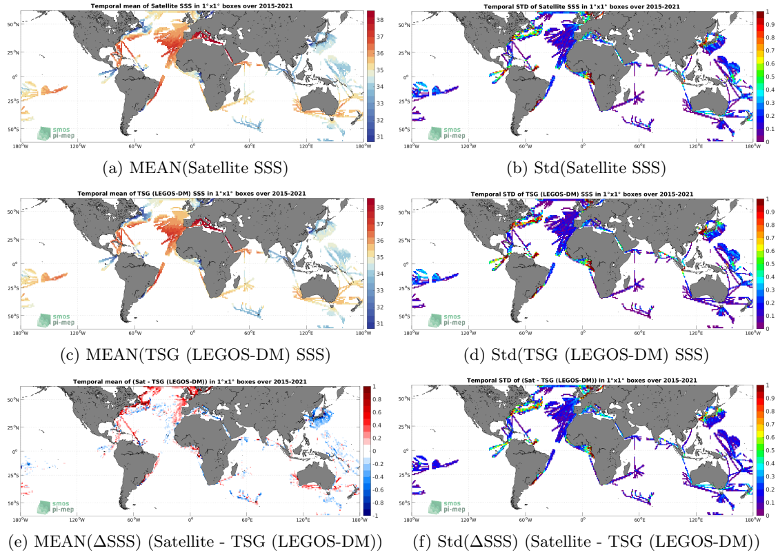
Figure 6: Temporal mean (left) and Std (right) of SSS from SMAP SSS L3 v5 - Monthly (RSS) (top), TSG (LEGOS-DM) (middle), and of \Delta SSS (Satellite - TSG (LEGOS-DM)). Only match-up pairs are used to generate these maps.
