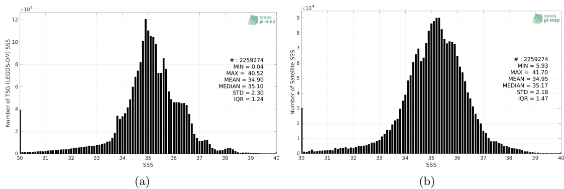
Figure 2: Histograms of SSS from TSG (LEGOS-DM) (a) and SMAP SSS L3 v5 - Monthly (RSS) (b) considering all match-up pairs per bins of 0.1 over the SMOS coastal zone (<800km) 60N-60S Pi-MEP region and for the full satellite product period.
