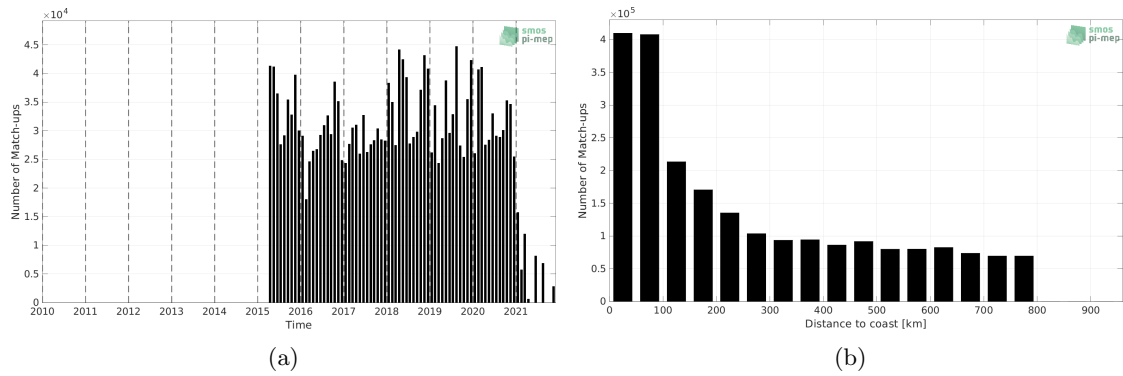
Figure 1: Number of match-ups between TSG (LEGOS-DM) and SMAP SSS L3 v5 - Monthly (RSS) SSS as a function of time (a) and as function of the distance to coast (b) over the SMOS coastal zone (<800km) 60N-60S Pi-MEP region and for the full satellite product period.
