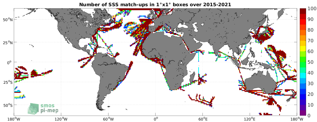
Figure 4: Number of SSS match-ups between TSG (LEGOS-DM) SSS and the SMAP SSS L3 v5 - Monthly (RSS) SSS product for the SMOS coastal zone (<800km) 60N-60S Pi-MEP region over 1^\circ \times 1^\circ boxes and for the full satellite product period.
