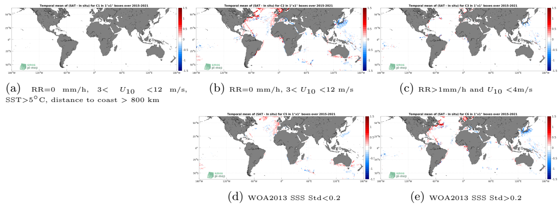
Figure 12: Temporal mean gridded over spatial boxes of size 1^\circ \times 1^\circ of \Delta SSS (SMAP SSS L3 v5 - Monthly (RSS) - TSG (LEGOS-DM)) for 5 different subdatasets corresponding to:RR=0 mm/h, 3 < U_{10} < 12 m/s, SST >5^\circ\text{C} , distance to coast > 800 km (a), RR=0 mm/h, 3 < U_{10} < 12 m/s (b), RR >1 mm/h and U_{10} < 4 m/s (c), WOA2013 SSS Std <0.2 (d), WOA2013 SSS Std >0.2 (e).
