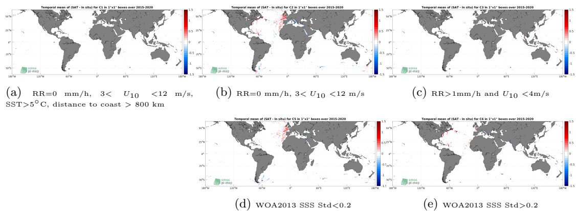
Figure 12: Temporal mean gridded over spatial boxes of size 1^\circ \times 1^\circ of \Delta SSS (SMAP SSS L3 v5 - Monthly (RSS) - TSG (GOSUD-Sailing-ship)) for 5 different subdatasets corresponding to:RR=0 mm/h, 3 < U_{10} < 12 m/s, SST >5^\circ\text{C} , distance to coast > 800 km (a), RR=0 mm/h, 3 < U_{10} < 12 m/s (b), RR >1 mm/h and U_{10} < 4 m/s (c), WOA2013 SSS Std <0.2 (d), WOA2013 SSS Std >0.2 (e).
