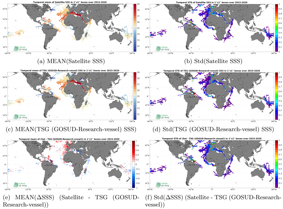
Figure 6: Temporal mean (left) and Std (right) of SSS from SMAP SSS L3 v5 - Monthly (RSS) (top), TSG (GOSUD-Research-vessel) (middle), and of \Delta SSS (Satellite - TSG (GOSUD-Research-vessel)). Only match-up pairs are used to generate these maps.
