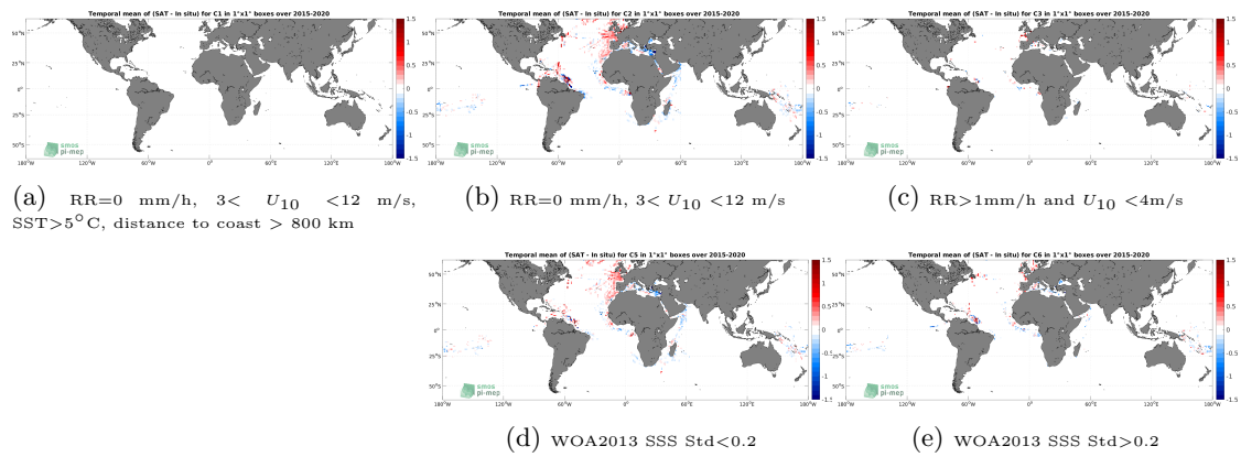
Figure 12: Temporal mean gridded over spatial boxes of size 1^\circ \times 1^\circ of \Delta\text{SSS} (SMAP SSS L3 v5 - Monthly (RSS) - TSG (GOSUD-Research-vessel)) for 5 different subdatasets corresponding to:RR=0 mm/h, 3 < U_{10} < 12 m/s, SST >5^\circ\text{C} , distance to coast > 800 km (a), RR=0 mm/h, 3 < U_{10} < 12 m/s (b), RR >1 mm/h and U_{10} < 4 m/s (c), WOA2013 SSS Std <0.2 (d), WOA2013 SSS Std >0.2 (e).
