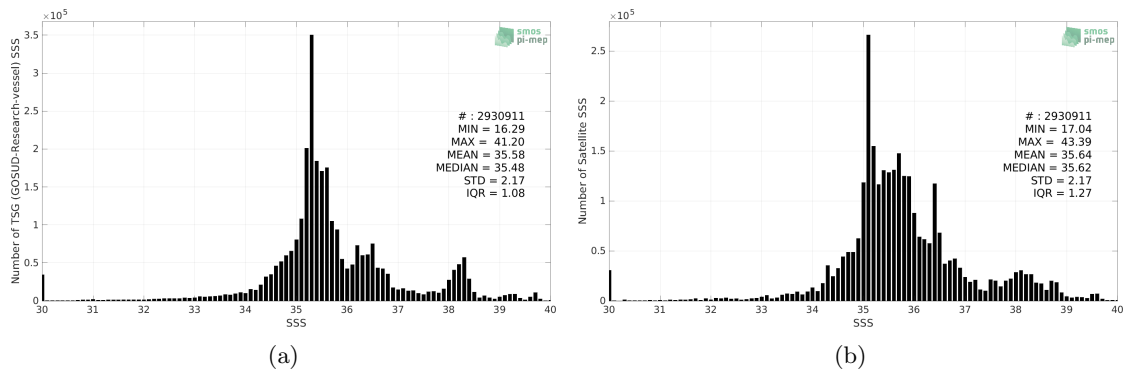
Figure 2: Histograms of SSS from TSG (GOSUD-Research-vessel) (a) and SMAP SSS L3 v5 - Monthly (RSS) (b) considering all match-up pairs per bins of 0.1 over the SMOS coastal zone (<800km) 60N-60S Pi-MEP region and for the full satellite product period.
