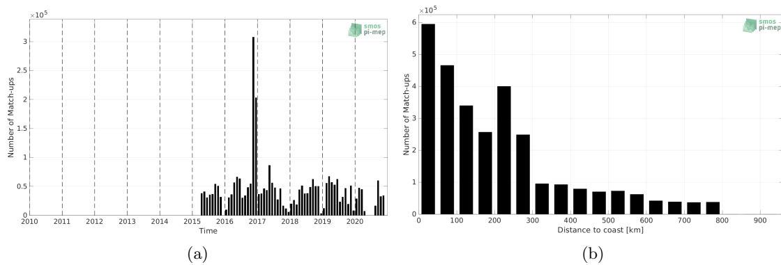
Figure 1: Number of match-ups between TSG (GOSUD-Research-vessel) and SMAP SSS L3 v5 - Monthly (RSS) SSS as a function of time (a) and as function of the distance to coast (b) over the SMOS coastal zone (<800km) 60N-60S Pi-MEP region and for the full satellite product period.
