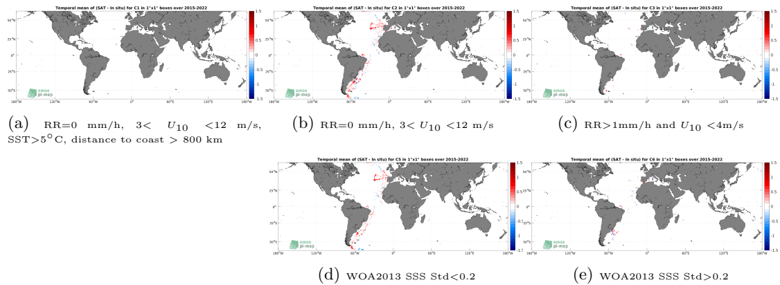
Figure 12: Temporal mean gridded over spatial boxes of size 1^\circ \times 1^\circ of \Delta SSS (SMAP SSS L3 v5 - Monthly (RSS) - TSG (CSIC-UTM)) for 5 different subdatasets corresponding to:RR=0 mm/h, 3 < U_{10} < 12 m/s, SST >5^\circ\text{C} , distance to coast > 800 km (a), RR=0 mm/h, 3 < U_{10} < 12 m/s (b), RR >1 mm/h and U_{10} < 4 m/s (c), WOA2013 SSS Std <0.2 (d), WOA2013 SSS Std >0.2 (e).
