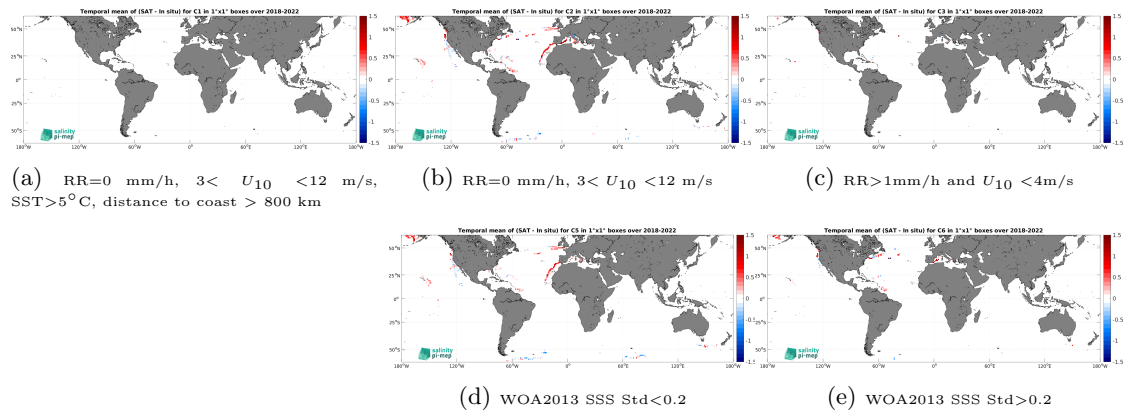
Figure 12: Temporal mean gridded over spatial boxes of size 1^\circ \times 1^\circ of \Delta\text{SSS} (SMAP SSS L3 v5 - Monthly (RSS) - Saildrone) for 5 different subdatasets corresponding to:RR=0 mm/h, 3 < U_{10} < 12 m/s, SST >5^\circ\text{C} , distance to coast > 800 km (a), RR=0 mm/h, 3 < U_{10} < 12 m/s (b), RR >1 mm/h and U_{10} < 4 m/s (c), WOA2013 SSS Std <0.2 (d), WOA2013 SSS Std >0.2 (e).
