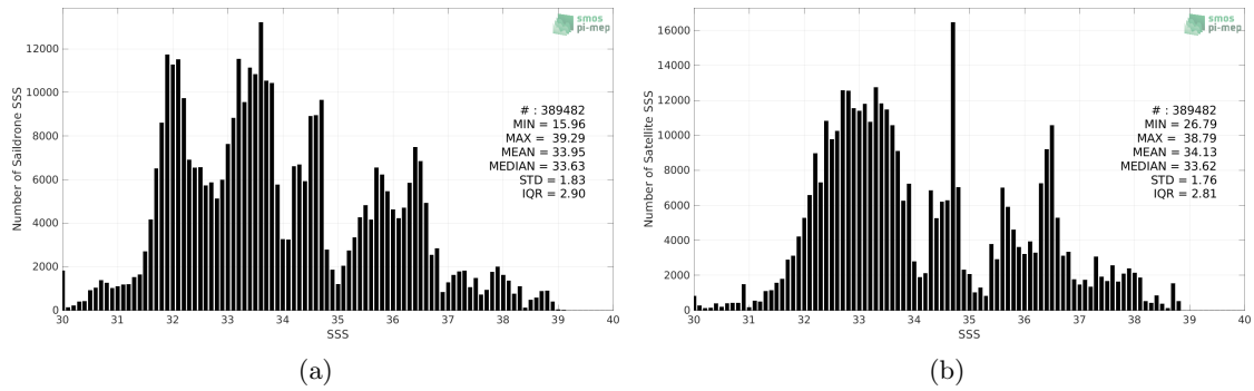
Figure 2: Histograms of SSS from Saildrone (a) and SMAP SSS L3 v5 - Monthly (RSS) (b) considering all match-up pairs per bins of 0.1 over the SMOS coastal zone (<800km) 60N-60S Pi-MEP region and for the full satellite product period.
