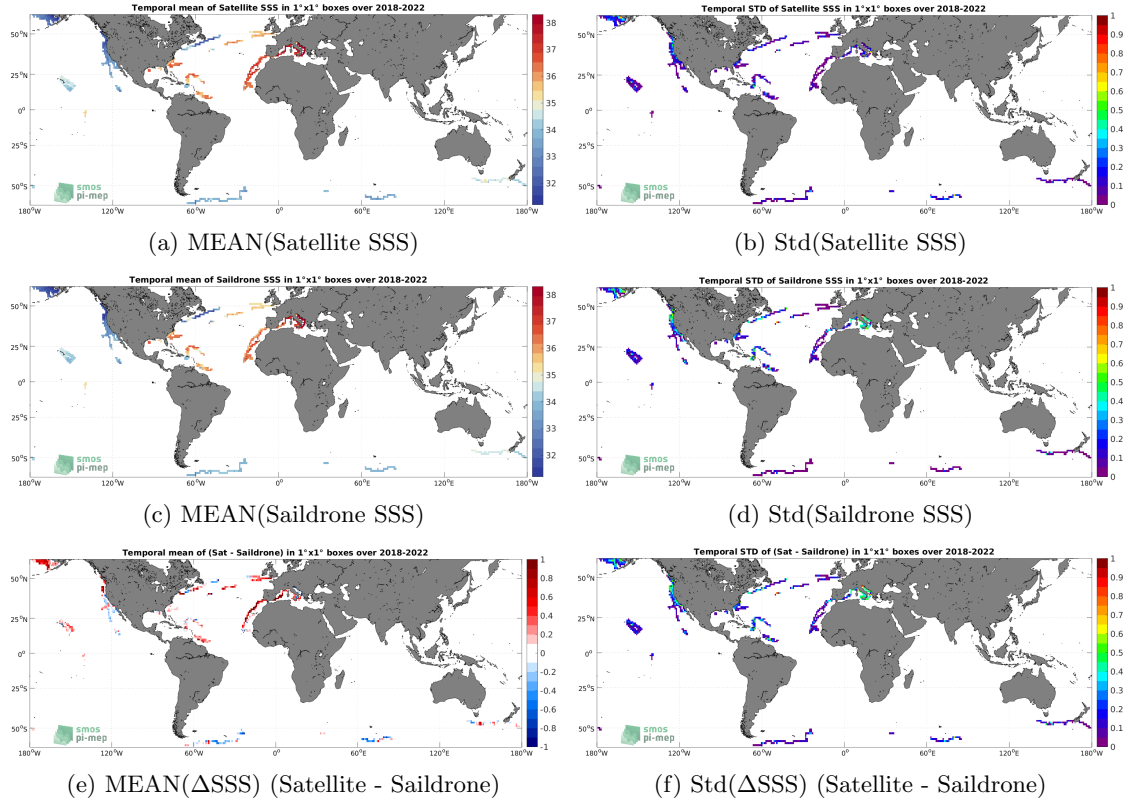
Figure 6: Temporal mean (left) and Std (right) of SSS from SMAP SSS L3 v5 - Monthly (RSS) (top), Saildrone (middle), and of \Delta SSS (Satellite - Saildrone). Only match-up pairs are used to generate these maps.
