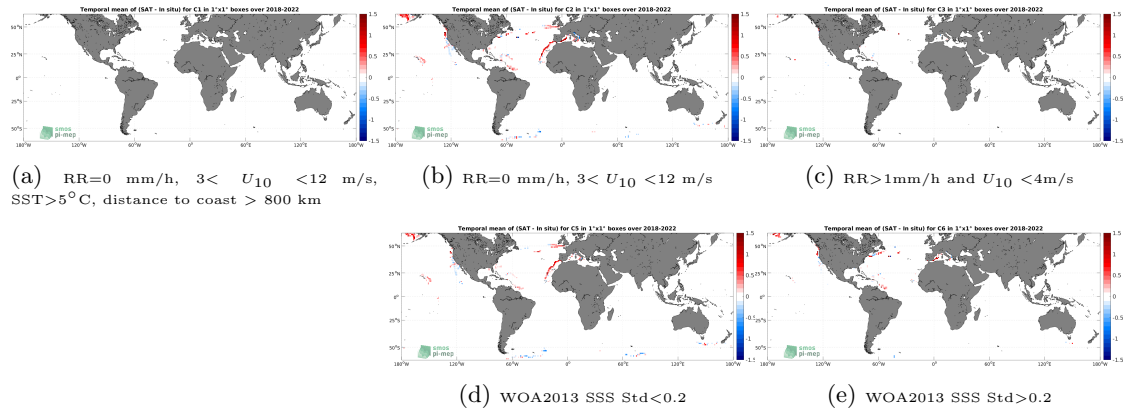
Figure 12: Temporal mean gridded over spatial boxes of size 1^\circ \times 1^\circ of \Delta SSS (SMAP SSS L3 v5 - Monthly (RSS) - Saildrone) for 5 different subdatasets corresponding to:RR=0 mm/h, 3 < U_{10} < 12 m/s, SST >5^\circ\text{C} , distance to coast > 800 km (a), RR=0 mm/h, 3 < U_{10} < 12 m/s (b), RR >1 mm/h and U_{10} < 4 m/s (c), WOA2013 SSS Std <0.2 (d), WOA2013 SSS Std >0.2 (e).
