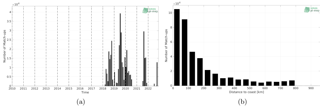
Figure 1: Number of match-ups between Saildrone and SMAP SSS L3 v5 - Monthly (RSS) SSS as a function of time (a) and as function of the distance to coast (b) over the SMOS coastal zone (<800km) 60N-60S Pi-MEP region and for the full satellite product period.
