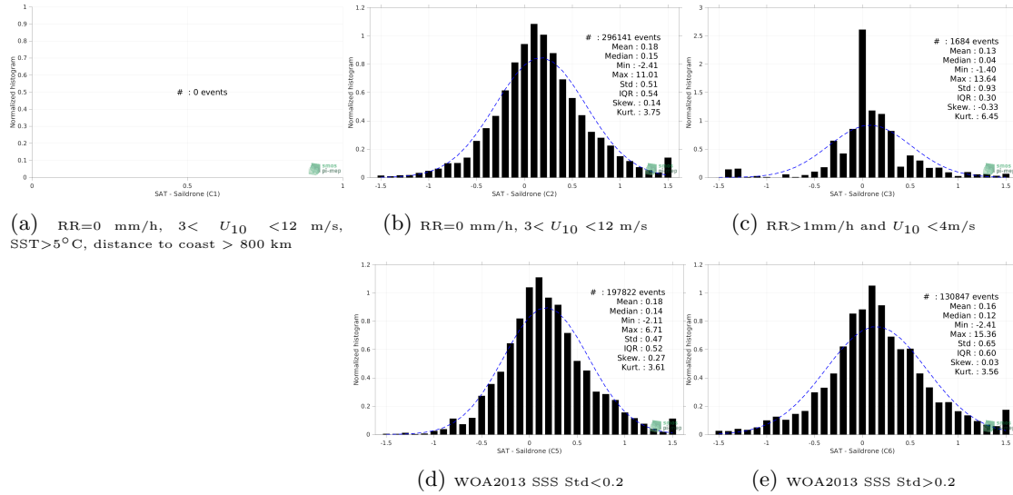
Figure 13: Normalized histogram of \Delta SSS (SMAP SSS L3 v5 - Monthly (RSS) - Saildrone) for 5 different subdatasets corresponding to: RR=0 mm/h, 3 < U_{10} < 12 m/s, SST > 5°C, distance to coast > 800 km (a), RR=0 mm/h, 3 < U_{10} < 12 m/s (b), RR > 1mm/h and U_{10} < 4 m/s (c), WOA2013 SSS Std < 0.2 (d), WOA2013 SSS Std > 0.2 (e).
