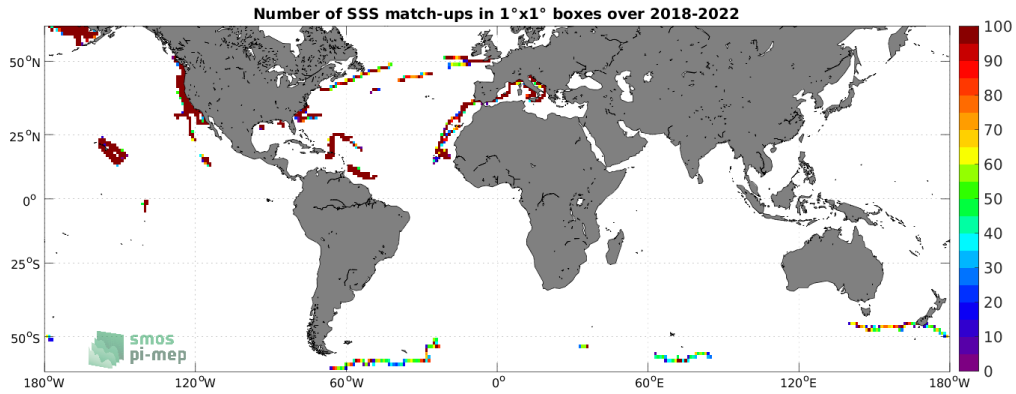
Figure 4: Number of SSS match-ups between Saildrone SSS and the SMAP SSS L3 v5 - Monthly (RSS) SSS product for the SMOS coastal zone (<800km) 60N-60S Pi-MEP region over 1^\circ \times 1^\circ boxes and for the full satellite product period.
