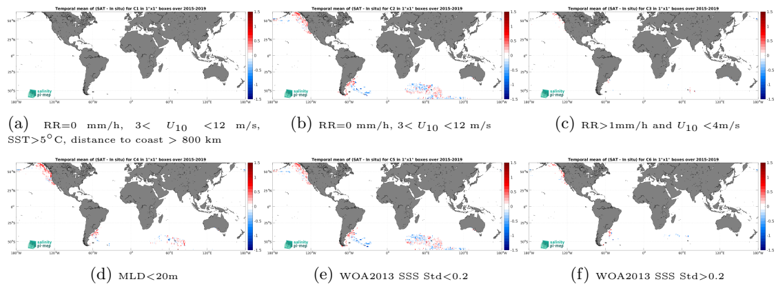
Figure 12: Temporal mean gridded over spatial boxes of size 1^\circ \times 1^\circ of \Delta SSS (SMAP SSS L3 v5 - Monthly (RSS) - Marine mammals) for 6 different subdatasets corresponding to:RR=0 mm/h, 3 < U_{10} < 12 m/s, SST >5^\circ C, distance to coast > 800 km (a), RR=0 mm/h, 3 < U_{10} < 12 m/s (b), RR >1 mm/h and U_{10} < 4 m/s (c),MLD <20 m (d),WOA2013 SSS Std <0.2 (e),WOA2013 SSS Std >0.2 (f).
