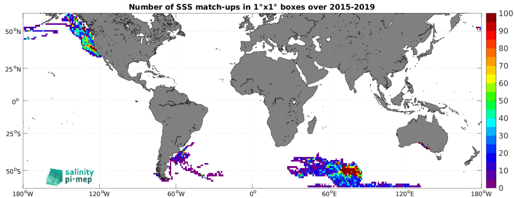
Figure 4: Number of SSS match-ups between Marine mammals SSS and the SMAP SSS L3 v5 - Monthly (RSS) SSS product for the SMOS coastal zone (<800km) 60N-60S Pi-MEP region over 1^\circ \times 1^\circ boxes and for the full satellite product period.
