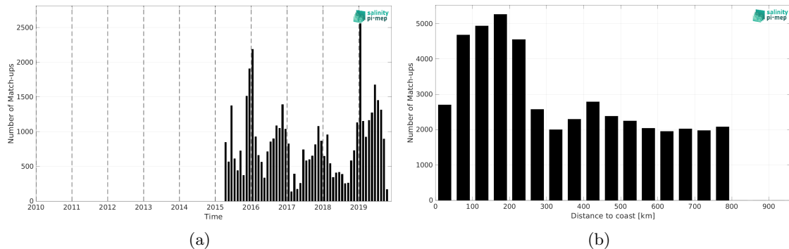
Figure 1: Number of match-ups between Marine mammals and SMAP SSS L3 v5 - Monthly (RSS) SSS as a function of time (a) and as function of the distance to coast (b) over the SMOS coastal zone (<800km) 60N-60S Pi-MEP region and for the full satellite product period.
