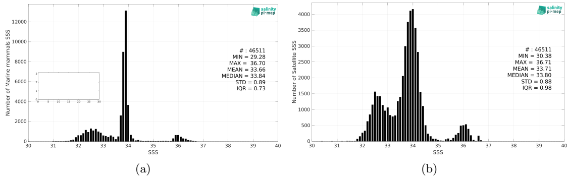
Figure 2: Histograms of SSS from Marine mammals (a) and SMAP SSS L3 v5 - Monthly (RSS) (b) considering all match-up pairs per bins of 0.1 over the SMOS coastal zone (<800km) 60N-60S Pi-MEP region and for the full satellite product period.
