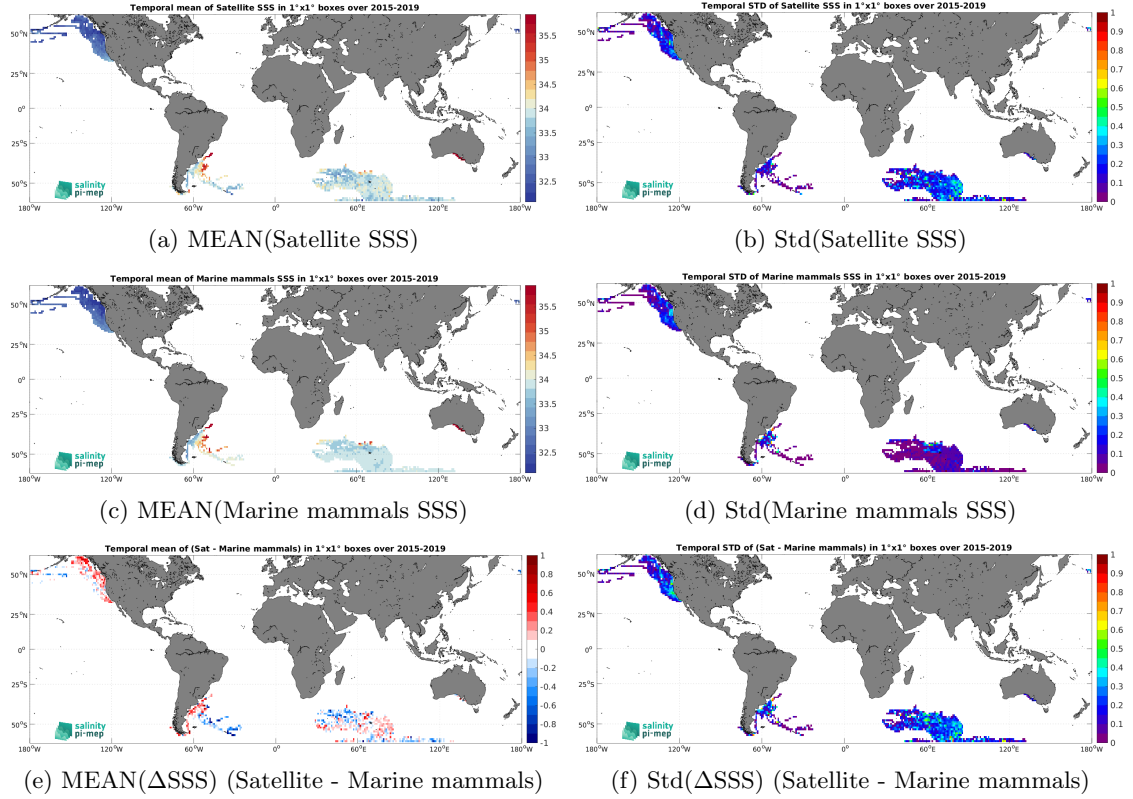
Figure 6: Temporal mean (left) and Std (right) of SSS from SMAP SSS L3 v5 - Monthly (RSS) (top), Marine mammals (middle), and of \Delta SSS (Satellite - Marine mammals). Only match-up pairs are used to generate these maps.
