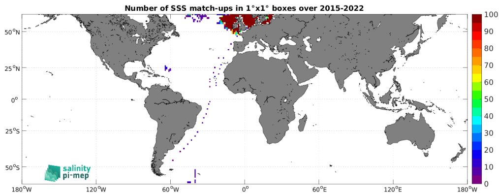
Figure 4: Number of SSS match-ups between ICES SSS and the SMAP SSS L3 v5 - Monthly (RSS) SSS product for the SMOS coastal zone (<800km) 60N-60S Pi-MEP region over 1^\circ \times 1^\circ boxes and for the full satellite product period.
