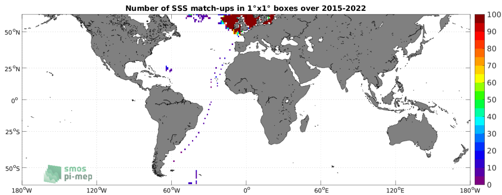
Figure 4: Number of SSS match-ups between ICES SSS and the SMAP SSS L3 v5 - Monthly (RSS) SSS product for the SMOS coastal zone (<800km) 60N-60S Pi-MEP region over 1°×1° boxes and for the full satellite product period.
