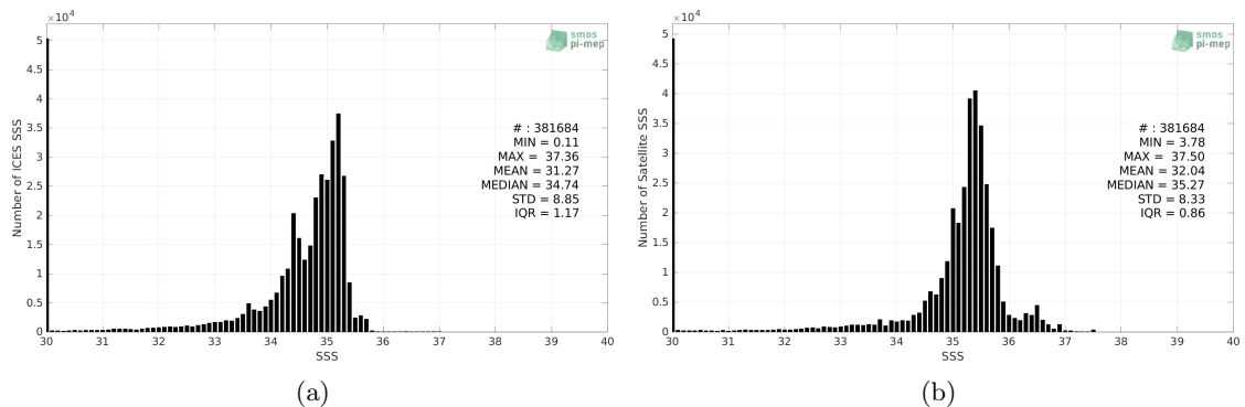
Figure 2: Histograms of SSS from ICES (a) and SMAP SSS L3 v5 - Monthly (RSS) (b) considering all match-up pairs per bins of 0.1 over the SMOS coastal zone (<800km) 60N-60S Pi-MEP region and for the full satellite product period.
