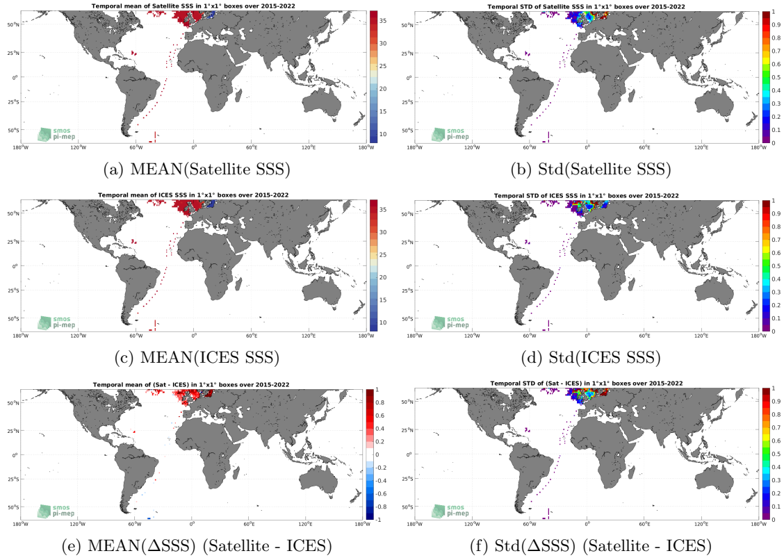
Figure 6: Temporal mean (left) and Std (right) of SSS from SMAP SSS L3 v5 - Monthly (RSS) (top), ICES (middle), and of \Delta SSS (Satellite - ICES). Only match-up pairs are used to generate these maps.
