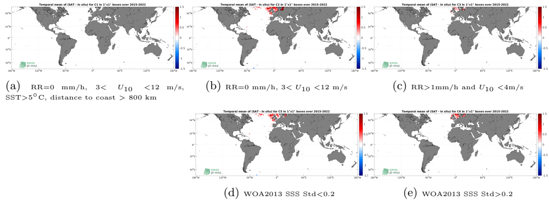
Figure 12: Temporal mean gridded over spatial boxes of size 1^\circ \times 1^\circ of \Delta SSS (SMAP SSS L3 v5 - Monthly (RSS) - ICES) for 5 different subdatasets corresponding to:RR=0 mm/h, 3 < U_{10} < 12 m/s, SST >5^\circ\text{C} , distance to coast > 800 km (a), RR=0 mm/h, 3 < U_{10} < 12 m/s (b), RR >1 mm/h and U_{10} < 4 m/s (c), WOA2013 SSS Std <0.2 (d), WOA2013 SSS Std >0.2 (e).
