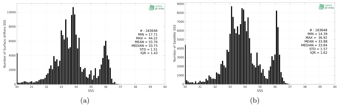
Figure 2: Histograms of SSS from Surface drifters (a) and SMAP SSS L3 v5 - Monthly (RSS) (b) considering all match-up pairs per bins of 0.1 over the SMOS coastal zone (<800km) 60N-60S Pi-MEP region and for the full satellite product period.
