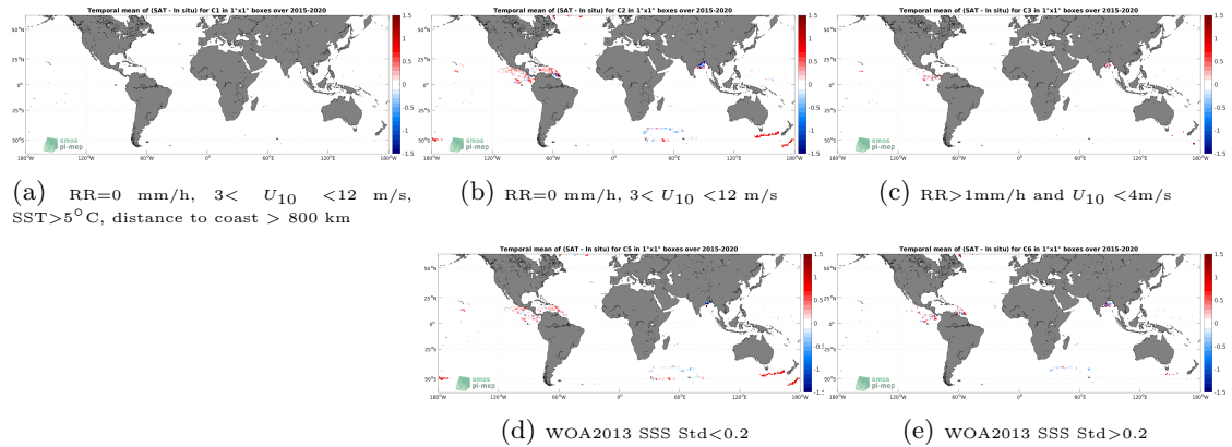
Figure 11: Temporal mean gridded over spatial boxes of size 1^\circ \times 1^\circ of \Delta SSS (SMAP SSS L3 v5 - Monthly (RSS) - Surface drifters) for 5 different subdatasets corresponding to:RR=0 mm/h, 3 < U_{10} < 12 m/s, SST >5^\circ\text{C} , distance to coast > 800 km (a), RR=0 mm/h, 3 < U_{10} < 12 m/s (b), RR >1 mm/h and U_{10} < 4 m/s (c), WOA2013 SSS Std <0.2 (d), WOA2013 SSS Std >0.2 (e).
