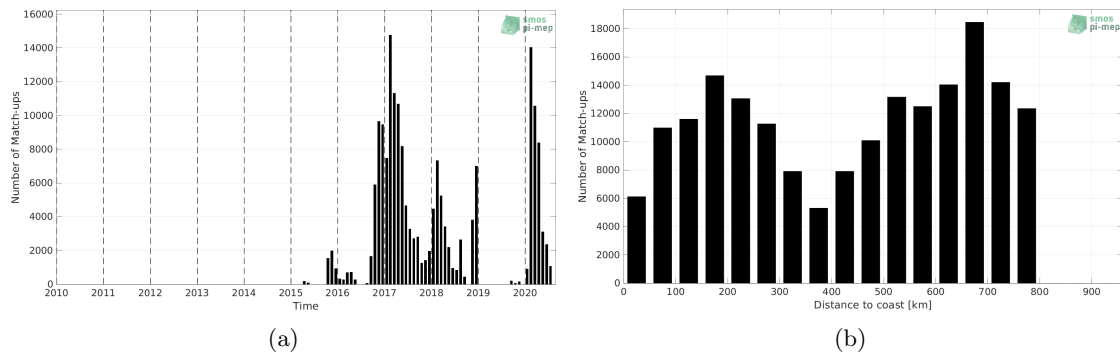
Figure 1: Number of match-ups between Surface drifters and SMAP SSS L3 v5 - Monthly (RSS) SSS as a function of time (a) and as function of the distance to coast (b) over the SMOS coastal zone (<800km) 60N-60S Pi-MEP region and for the full satellite product period.
