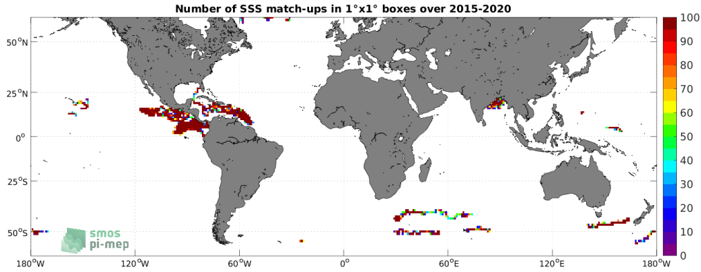
Figure 3: Number of SSS match-ups between Surface drifters SSS and the SMAP SSS L3 v5 - Monthly (RSS) SSS product for the SMOS coastal zone (<800km) 60N-60S Pi-MEP region over 1^\circ \times 1^\circ boxes and for the full satellite product period.
