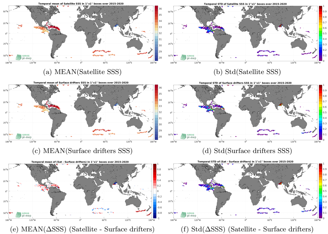
Figure 5: Temporal mean (left) and Std (right) of SSS from SMAP SSS L3 v5 - Monthly (RSS) (top), Surface drifters (middle), and of \Delta SSS (Satellite - Surface drifters). Only match-up pairs are used to generate these maps.
