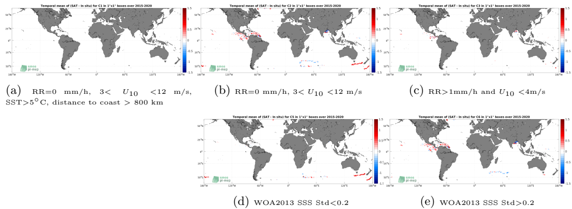
Figure 11: Temporal mean gridded over spatial boxes of size 1^\circ \times 1^\circ of \Delta\text{SSS} (SMAP SSS L3 v5 - Monthly (RSS) - Surface drifters) for 5 different subdatasets corresponding to: \text{RR}=0 mm/h, 3 < U_{10} < 12 m/s, \text{SST} > 5^\circ\text{C} , distance to coast > 800 km (a), \text{RR}=0 mm/h, 3 < U_{10} < 12 m/s (b), \text{RR} > 1\text{mm/h} and U_{10} < 4\text{m/s} (c), WOA2013 SSS Std < 0.2 (d), WOA2013 SSS Std > 0.2 (e).
