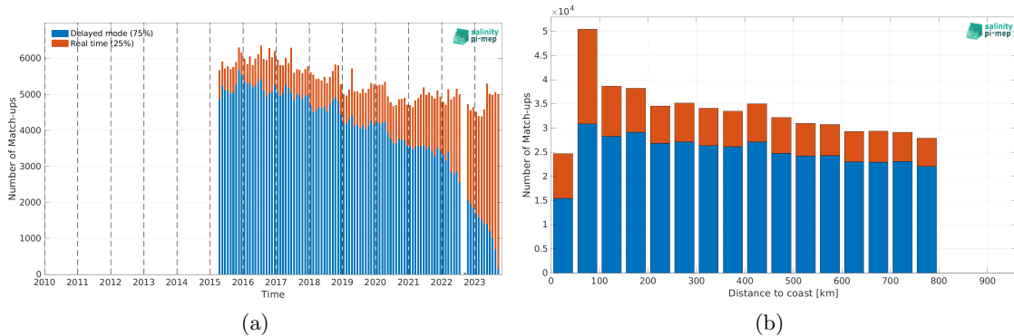
Figure 1: Number of match-ups between Argo and SMAP SSS L3 v5 - Monthly (RSS) SSS as a function of time (a) and as function of the distance to coast (b) over the SMOS coastal zone (<800km) 60N-60S Pi-MEP region and for the full satellite product period.
