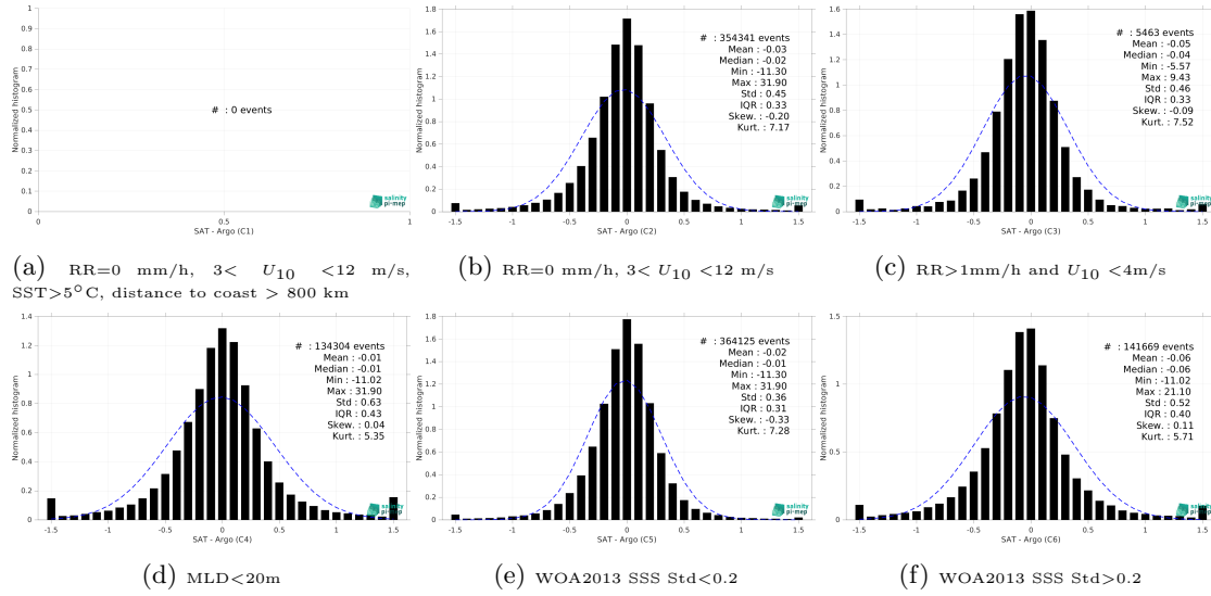
Figure 13: Normalized histogram of \Delta\text{SSS} (SMAP SSS L3 v5 - Monthly (RSS) - Argo) for 6 different subdatasets corresponding to: RR=0 mm/h, 3 < U_{10} < 12 m/s, SST>5°C, distance to coast > 800 km (a), RR=0 mm/h, 3 < U_{10} < 12 m/s (b), RR>1mm/h and U_{10} < 4 m/s (c), MLD<20m (d), WOA2013 SSS Std<0.2 (e), WOA2013 SSS Std>0.2 (f).
