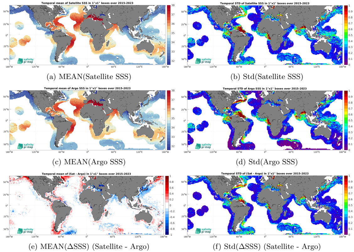
Figure 6: Temporal mean (left) and Std (right) of SSS from SMAP SSS L3 v5 - Monthly (RSS) (top), Argo (middle), and of \Delta SSS (Satellite - Argo). Only match-up pairs are used to generate these maps.
