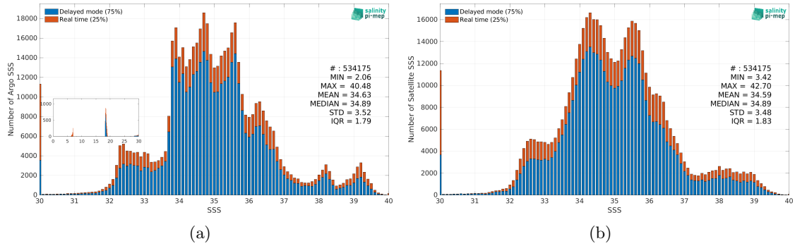
Figure 2: Histograms of SSS from Argo (a) and SMAP SSS L3 v5 - Monthly (RSS) (b) considering all match-up pairs per bins of 0.1 over the SMOS coastal zone (<800km) 60N-60S Pi-MEP region and for the full satellite product period.
