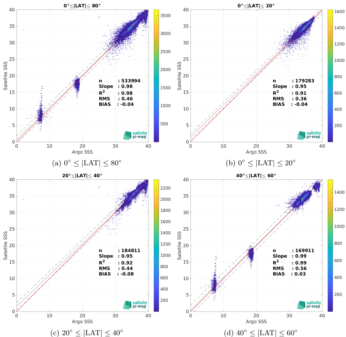
Figure 9: Contour maps of the concentration of SMAP SSS L3 v5 - Monthly (RSS) SSS (y-axis) versus Argo SSS (x-axis) at match-up pairs for different latitude bands. For each plot, the red line shows x=y . The black thin and dashed lines indicate a linear fit through the data cloud and the \pm 95\% confidence levels, respectively. The number match-up pairs n , the slope and R^2 coefficient of the linear fit, the root mean square (RMS) and the mean bias between satellite and in situ data are indicated for each latitude band in each plots.
