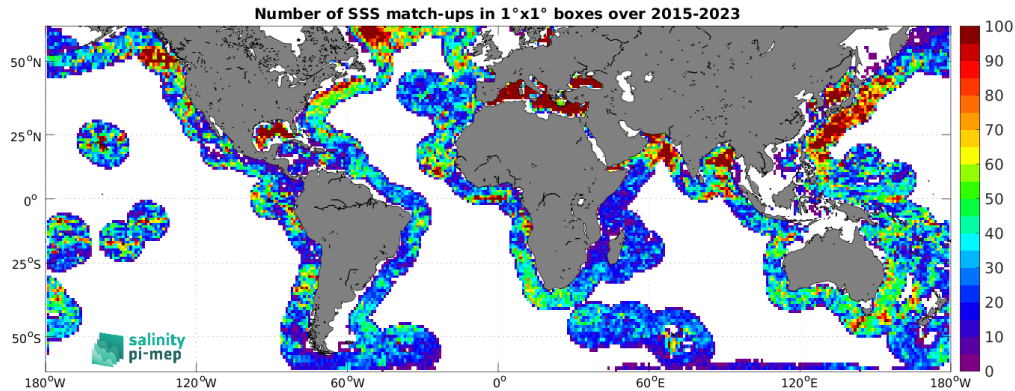
Figure 4: Number of SSS match-ups between Argo SSS and the SMAP SSS L3 v5 - Monthly (RSS) SSS product for the SMOS coastal zone (<800km) 60N-60S Pi-MEP region over 1^\circ \times 1^\circ boxes and for the full satellite product period.
