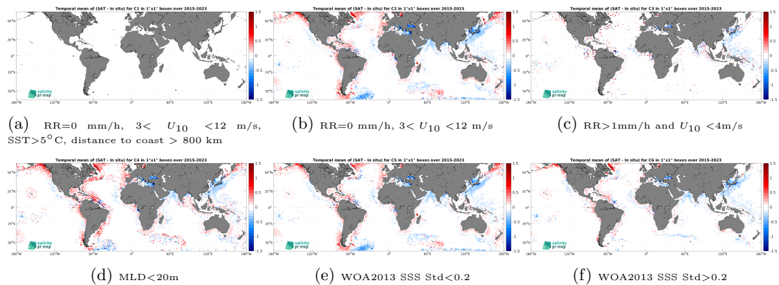
Figure 12: Temporal mean gridded over spatial boxes of size 1^\circ \times 1^\circ of \Delta SSS (SMAP SSS L3 v5 - Monthly (RSS) - Argo) for 6 different subdatasets corresponding to:RR=0 mm/h, 3 < U_{10} < 12 m/s, SST >5^\circ C, distance to coast > 800 km (a), RR=0 mm/h, 3 < U_{10} < 12 m/s (b), RR >1 mm/h and U_{10} < 4 m/s (c),MLD <20 m (d),WOA2013 SSS Std <0.2 (e),WOA2013 SSS Std >0.2 (f).
