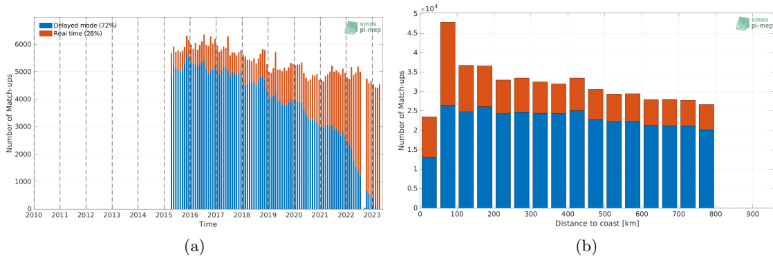
Figure 1: Number of match-ups between Argo and SMAP SSS L3 v5 - Monthly (RSS) SSS as a function of time (a) and as function of the distance to coast (b) over the SMOS coastal zone ( < 800\text{km} ) 60N-60S Pi-MEP region and for the full satellite product period.
