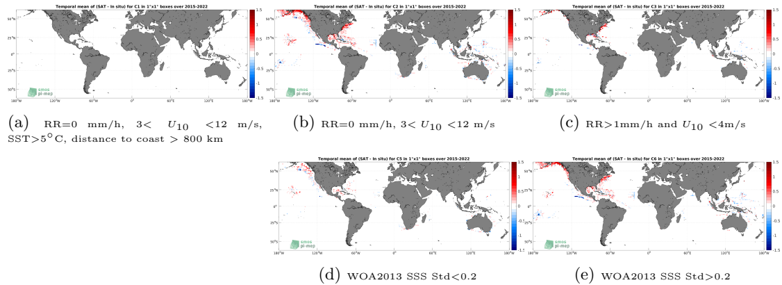
Figure 12: Temporal mean gridded over spatial boxes of size 1^\circ \times 1^\circ of \Delta\text{SSS} (SMAP SSS L3 v4 - 8-Day running (RSS) - TSG (SAMOS)) for 5 different subdatasets corresponding to:RR=0 mm/h, 3 < U_{10} < 12 m/s, SST >5^\circ\text{C} , distance to coast > 800 km (a), RR=0 mm/h, 3 < U_{10} < 12 m/s (b), RR >1 mm/h and U_{10} < 4 m/s (c), WOA2013 SSS Std <0.2 (d), WOA2013 SSS Std >0.2 (e).
