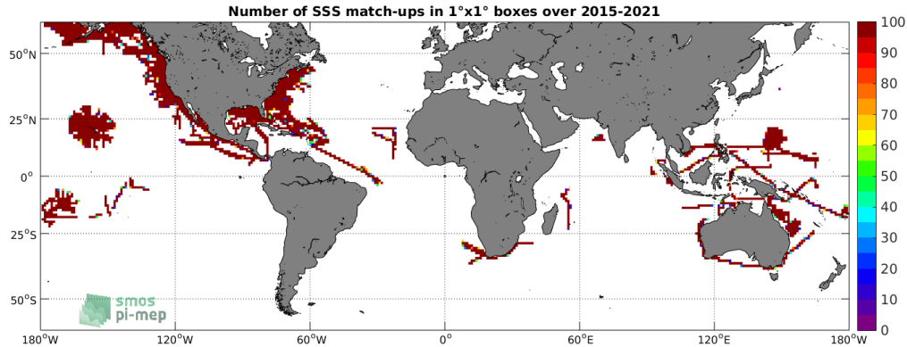
Figure 4: Number of SSS match-ups between TSG (SAMOS) SSS and the SMAP SSS L3 v4 - 8-Day running (RSS) SSS product for the SMOS coastal zone (<800km) 60N-60S Pi-MEP region over 1^\circ \times 1^\circ boxes and for the full satellite product period.
