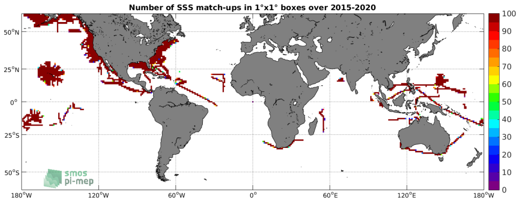
Figure 4: Number of SSS match-ups between TSG-SAMOS SSS and the SMAP-L3-RSS-V4-8DAY-RUNNING SSS product for the SMOS coastal zone (<800km) 60N-60S Pi-MEP region over 1^\circ \times 1^\circ boxes and for the full satellite product period.
