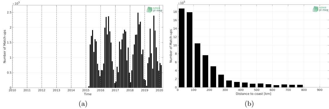
Figure 1: Number of match-ups between TSG-SAMOS and SMAP-L3-RSS-V4-8DAY-RUNNING SSS as a function of time (a) and as function of the distance to coast (b) over the SMOS coastal zone (<800km) 60N-60S Pi-MEP region and for the full satellite product period.
