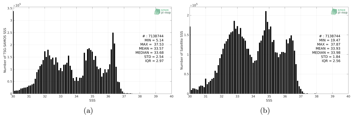
Figure 2: Histograms of SSS from TSG-SAMOS (a) and SMAP-L3-RSS-V4-8DAY-RUNNING (b) considering all match-up pairs per bins of 0.1 over the SMOS coastal zone (<800km) 60N-60S Pi-MEP region and for the full satellite product period.
