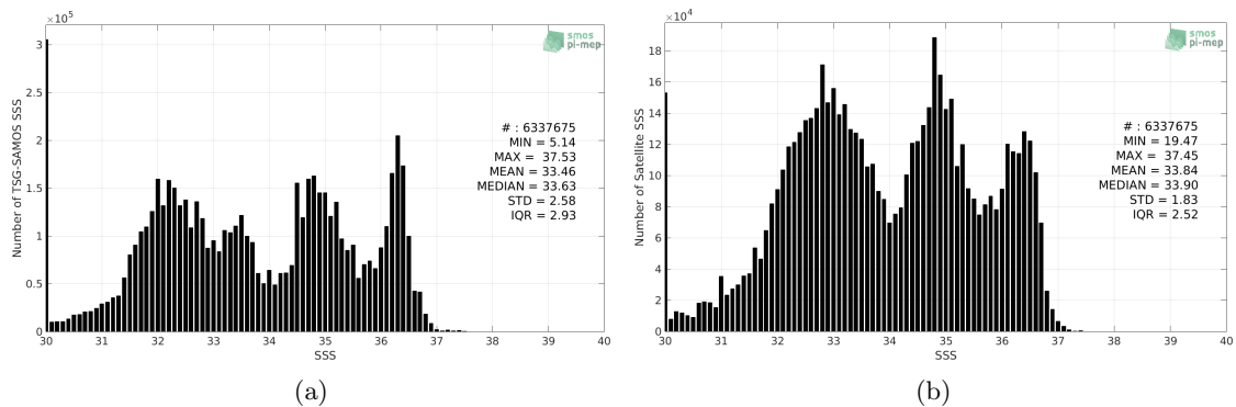
Figure 2: Histograms of SSS from TSG-SAMOS (a) and SMAP-L3-RSS-V4-8DAY-RUNNING (b) considering all match-up pairs per bins of 0.1 over the SMOS coastal zone ( \geq 800\text{km} ) 60N-60S Pi-MEP region and for the full satellite product period.
