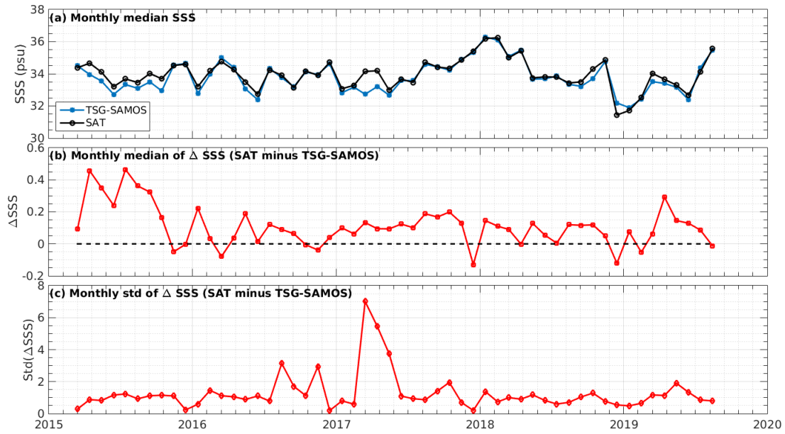
Figure 7: Time series of the monthly median SSS (top), median of \Delta SSS (Satellite - TSG-SAMOS) and Std of \Delta SSS (Satellite - TSG-SAMOS) over the SMOS coastal zone ( \leq 800 km) 60N-60S Pi-MEP region considering all match-ups collected by the Pi-MEP.
