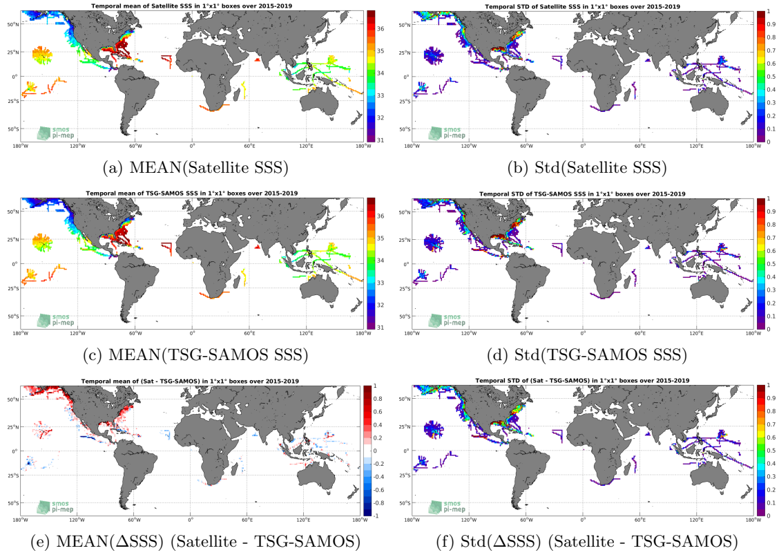
Figure 6: Temporal mean (left) and Std (right) of SSS from SMAP-L3-RSS-V4-8DAY-RUNNING (top), TSG-SAMOS (middle), and of \Delta SSS (Satellite - TSG-SAMOS). Only match-up pairs are used to generate these maps.
