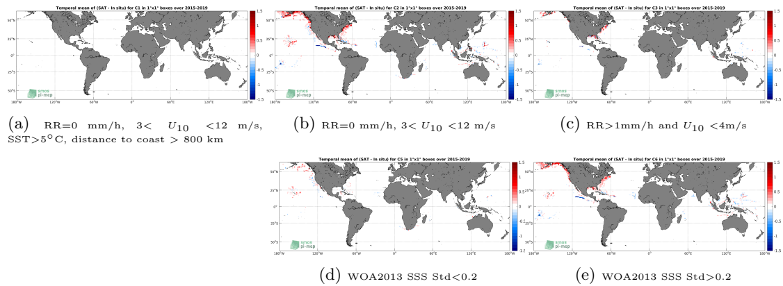
Figure 12: Temporal mean gridded over spatial boxes of size 1^\circ \times 1^\circ of \Delta SSS (SMAP-L3-RSS-V4-8DAY-RUNNING - TSG-SAMOS) for 5 different subdatasets corresponding to:RR=0 mm/h, 3 < U_{10} < 12 m/s, SST >5^\circ\text{C} , distance to coast > 800 km (a), RR=0 mm/h, 3 < U_{10} < 12 m/s (b), RR >1 mm/h and U_{10} < 4 m/s (c), WOA2013 SSS Std <0.2 (d), WOA2013 SSS Std >0.2 (e).
