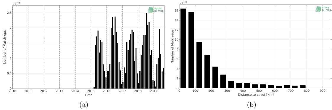
Figure 1: Number of match-ups between TSG-SAMOS and SMAP-L3-RSS-V4-8DAY-RUNNING SSS as a function of time (a) and as function of the distance to coast (b) over the SMOS coastal zone ( \geq 800\text{km} ) 60N-60S Pi-MEP region and for the full satellite product period.
