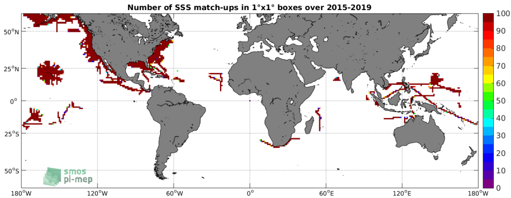
Figure 4: Number of SSS match-ups between TSG-SAMOS SSS and the SMAP-L3-RSS-V4-8DAY-RUNNING SSS product for the SMOS coastal zone ( \geq 800\text{km} ) 60N-60S Pi-MEP region over 1^\circ \times 1^\circ boxes and for the full satellite product period.
