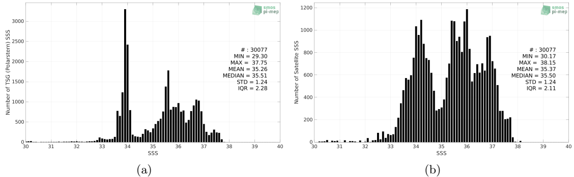
Figure 2: Histograms of SSS from TSG (Polarstern) (a) and SMAP SSS L3 v4 - 8-Day running (RSS) (b) considering all match-up pairs per bins of 0.1 over the SMOS coastal zone (<800km) 60N-60S Pi-MEP region and for the full satellite product period.
