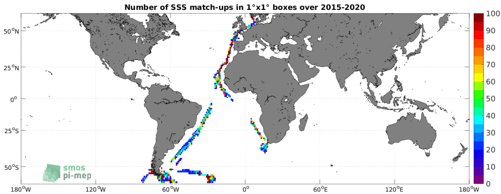
Figure 4: Number of SSS match-ups between TSG (Polarstern) SSS and the SMAP SSS L3 v4 - 8-Day running (RSS) SSS product for the SMOS coastal zone (<800km) 60N-60S Pi-MEP region over 1^\circ \times 1^\circ boxes and for the full satellite product period.
