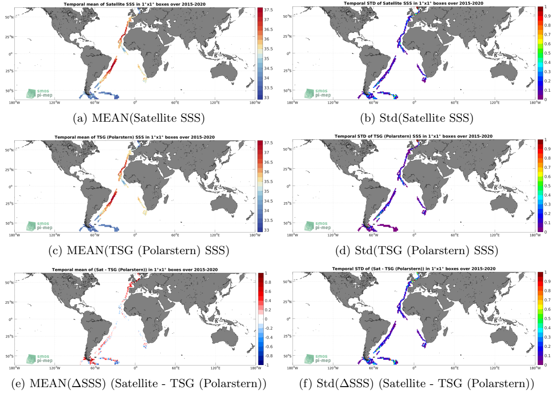
Figure 6: Temporal mean (left) and Std (right) of SSS from SMAP SSS L3 v4 - 8-Day running (RSS) (top), TSG (Polarstern) (middle), and of \Delta SSS (Satellite - TSG (Polarstern)). Only match-up pairs are used to generate these maps.
