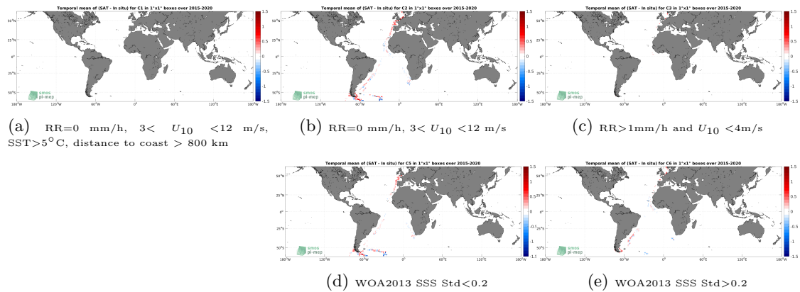
Figure 12: Temporal mean gridded over spatial boxes of size 1^\circ \times 1^\circ of \Delta SSS (SMAP SSS L3 v4 - 8-Day running (RSS) - TSG (Polarstern)) for 5 different subdatasets corresponding to:RR=0 mm/h, 3 < U_{10} < 12 m/s, SST >5^\circ\text{C} , distance to coast > 800 km (a), RR=0 mm/h, 3 < U_{10} < 12 m/s (b), RR >1 mm/h and U_{10} < 4 m/s (c), WOA2013 SSS Std <0.2 (d), WOA2013 SSS Std >0.2 (e).
