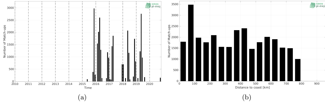
Figure 1: Number of match-ups between TSG (Polarstern) and SMAP SSS L3 v4 - 8-Day running (RSS) SSS as a function of time (a) and as function of the distance to coast (b) over the SMOS coastal zone (<800km) 60N-60S Pi-MEP region and for the full satellite product period.
