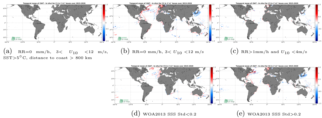
Figure 12: Temporal mean gridded over spatial boxes of size 1^\circ \times 1^\circ of \Delta SSS (SMAP SSS L3 v4 - 8-Day running (RSS) - TSG (LEGOS-DM)) for 5 different subdatasets corresponding to:RR=0 mm/h, 3 < U_{10} < 12 m/s, SST >5^\circ\text{C} , distance to coast > 800 km (a), RR=0 mm/h, 3 < U_{10} < 12 m/s (b), RR >1 mm/h and U_{10} < 4 m/s (c), WOA2013 SSS Std <0.2 (d), WOA2013 SSS Std >0.2 (e).
