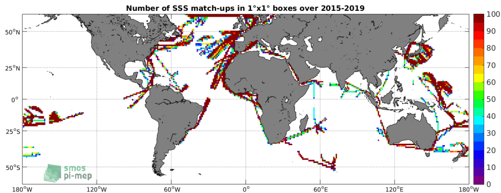
Figure 4: Number of SSS match-ups between TSG-LEGOS-DM SSS and the SMAP-L3-RSS-V4-8DAY-RUNNING SSS product for the SMOS coastal zone (<800km) 60N-60S Pi-MEP region over 1^\circ \times 1^\circ boxes and for the full satellite product period.
