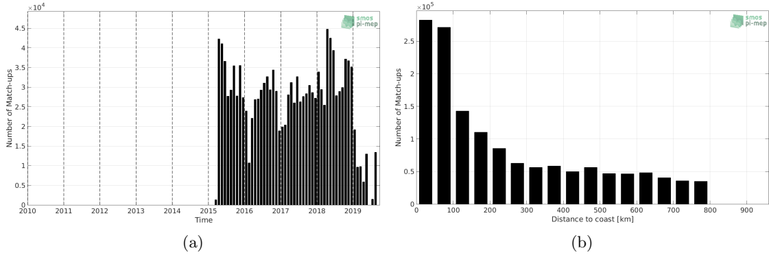
Figure 1: Number of match-ups between TSG-LEGOS-DM and SMAP-L3-RSS-V4-8DAY-RUNNING SSS as a function of time (a) and as function of the distance to coast (b) over the SMOS coastal zone (<800km) 60N-60S Pi-MEP region and for the full satellite product period.
