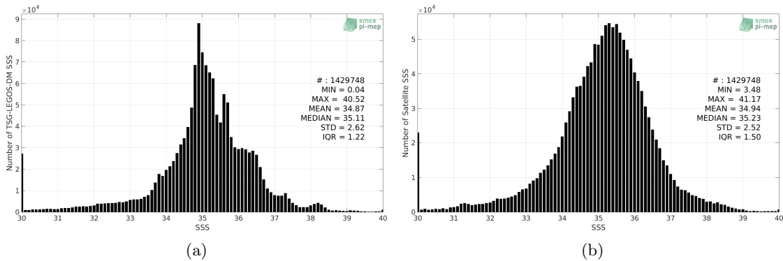
Figure 2: Histograms of SSS from TSG-LEGOS-DM (a) and SMAP-L3-RSS-V4-8DAY-RUNNING (b) considering all match-up pairs per bins of 0.1 over the SMOS coastal zone (<800km) 60N-60S Pi-MEP region and for the full satellite product period.
