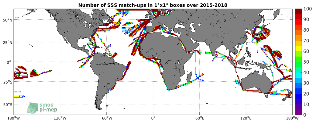
Figure 4: Number of SSS match-ups between TSG-LEGOS-DM SSS and the SMAP-L3-RSS-V4-8DAY-RUNNING SSS product for the SMOS coastal zone ( \pm 800\text{km} ) 60N-60S Pi-MEP region over 1^\circ \times 1^\circ boxes and for the full satellite product period.
