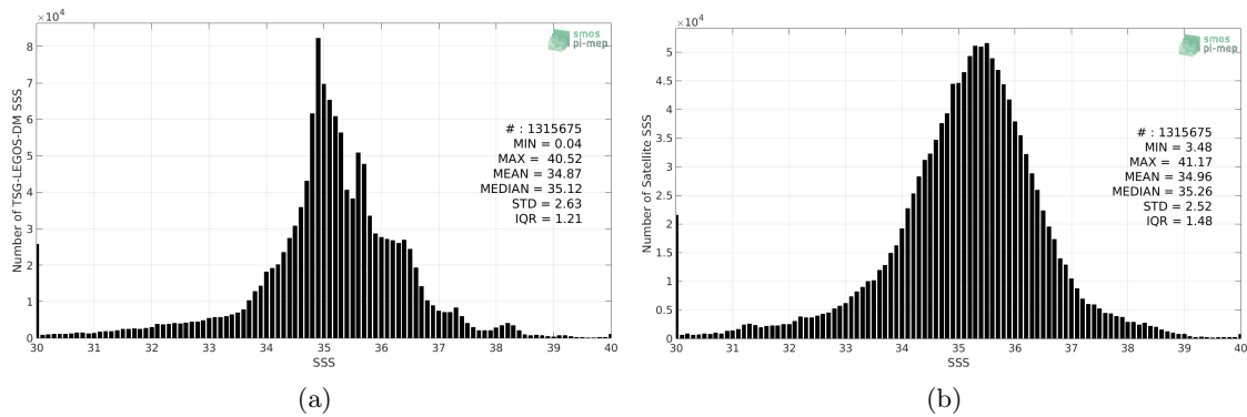
Figure 2: Histograms of SSS from TSG-LEGOS-DM (a) and SMAP-L3-RSS-V4-8DAY-RUNNING (b) considering all match-up pairs per bins of 0.1 over the SMOS coastal zone ( \leq 800 km) 60N-60S Pi-MEP region and for the full satellite product period.
