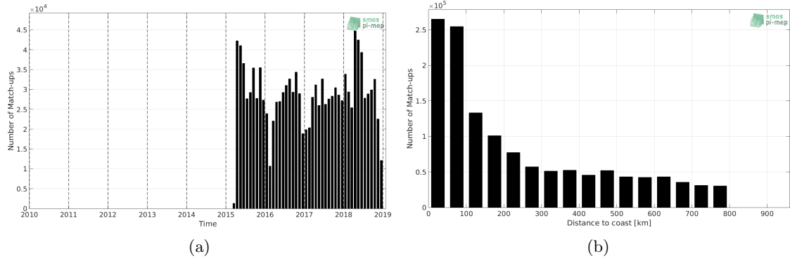
Figure 1: Number of match-ups between TSG-LEGOS-DM and SMAP-L3-RSS-V4-8DAY-RUNNING SSS as a function of time (a) and as function of the distance to coast (b) over the SMOS coastal zone ( \leq 800 km) 60N-60S Pi-MEP region and for the full satellite product period.
