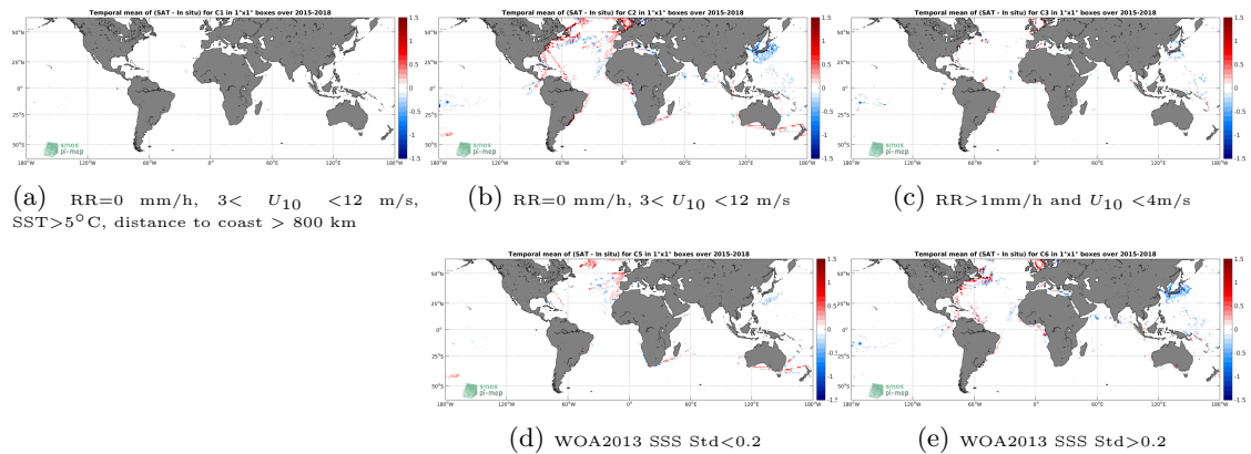
Figure 12: Temporal mean gridded over spatial boxes of size 1^\circ \times 1^\circ of \Delta SSS (SMAP-L3-RSS-V4-8DAY-RUNNING - TSG-LEGOS-DM) for 5 different subdatasets corresponding to:RR=0 mm/h, 3 < U_{10} < 12 m/s, SST > 5^\circ\text{C} , distance to coast > 800 km (a), RR=0 mm/h, 3 < U_{10} < 12 m/s (b), RR > 1 mm/h and U_{10} < 4 m/s (c), WOA2013 SSS Std < 0.2 (d), WOA2013 SSS Std > 0.2 (e).
