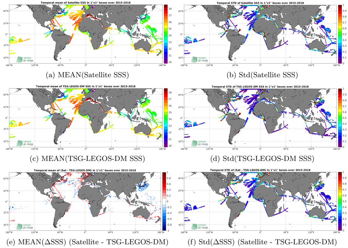
Figure 6: Temporal mean (left) and Std (right) of SSS from SMAP-L3-RSS-V4-8DAY-RUNNING (top), TSG-LEGOS-DM (middle), and of \Delta SSS (Satellite - TSG-LEGOS-DM). Only match-up pairs are used to generate these maps.
