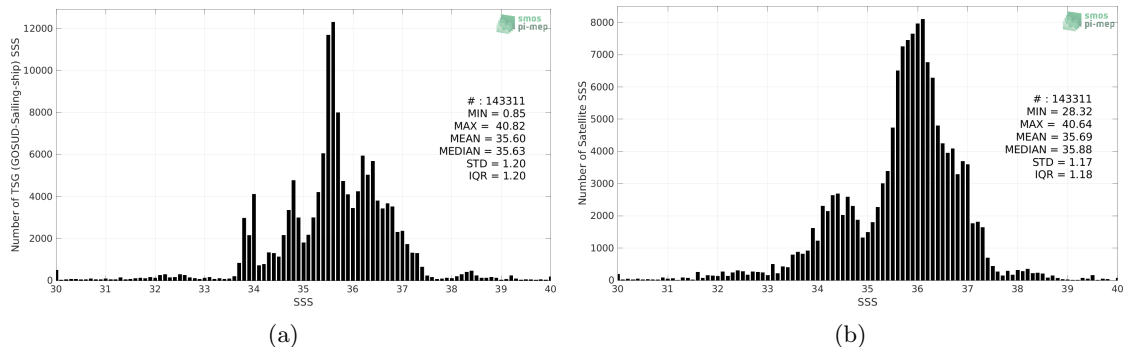
Figure 2: Histograms of SSS from TSG (GOSUD-Sailing-ship) (a) and SMAP SSS L3 v4 - 8-Day running (RSS) (b) considering all match-up pairs per bins of 0.1 over the SMOS coastal zone (<800km) 60N-60S Pi-MEP region and for the full satellite product period.
