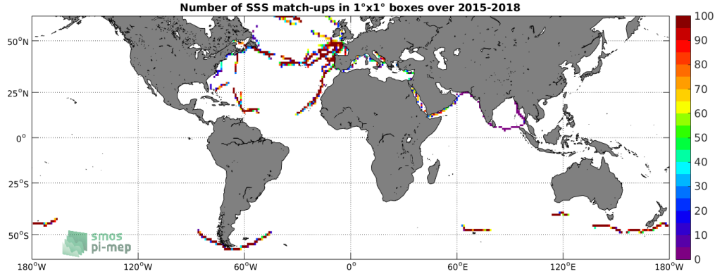
Figure 4: Number of SSS match-ups between TSG (GOSUD-Sailing-ship) SSS and the SMAP SSS L3 v4 - 8-Day running (RSS) SSS product for the SMOS coastal zone (<800km) 60N-60S Pi-MEP region over 1^\circ \times 1^\circ boxes and for the full satellite product period.
