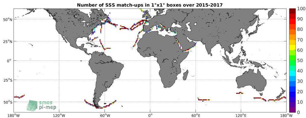
Figure 4: Number of SSS match-ups between TSG-GOSUD-Sailing-ship SSS and the SMAP-L3-RSS-V4-8DAY-RUNNING SSS product for the SMOS coastal zone (<800km) 60N-60S Pi-MEP region over 1°x1° boxes and for the full satellite product period.
