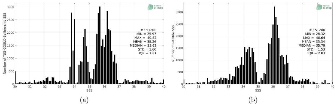
Figure 2: Histograms of SSS from TSG-GOSUD-Sailing-ship (a) and SMAP-L3-RSS-V4-8DAY-RUNNING (b) considering all match-up pairs per bins of 0.1 over the SMOS coastal zone (<800km) 60N-60S Pi-MEP region and for the full satellite product period.
