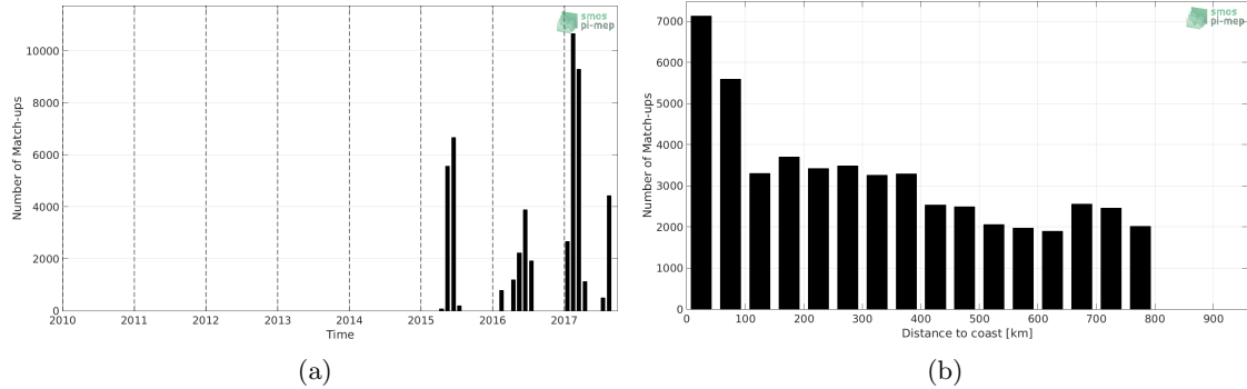
Figure 1: Number of match-ups between TSG-GOSUD-Sailing-ship and SMAP-L3-RSS-V4-8DAY-RUNNING SSS as a function of time (a) and as function of the distance to coast (b) over the SMOS coastal zone (<800km) 60N-60S Pi-MEP region and for the full satellite product period.
