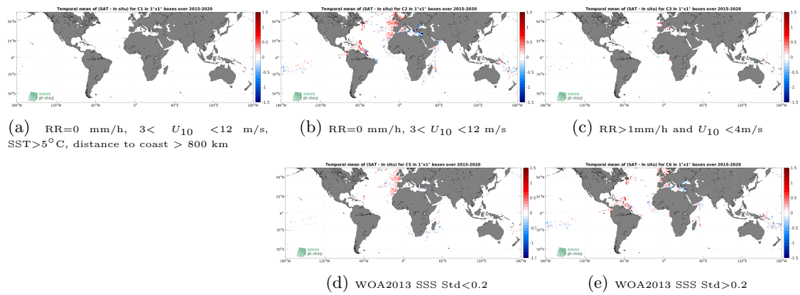
Figure 12: Temporal mean gridded over spatial boxes of size 1^\circ \times 1^\circ of \Delta\text{SSS} (SMAP SSS L3 v4 - 8-Day running (RSS) - TSG (GOSUD-Research-vessel)) for 5 different subdatasets corresponding to:RR=0 mm/h, 3 < U_{10} < 12 m/s, SST >5^\circ\text{C} , distance to coast > 800 km (a), RR=0 mm/h, 3 < U_{10} < 12 m/s (b), RR >1 mm/h and U_{10} < 4 m/s (c), WOA2013 SSS Std <0.2 (d), WOA2013 SSS Std >0.2 (e).
