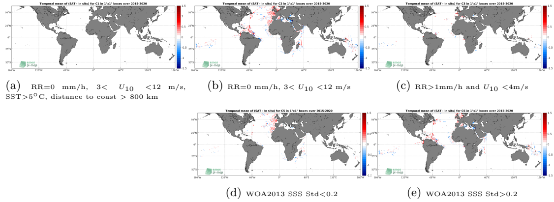
Figure 12: Temporal mean gridded over spatial boxes of size 1^\circ \times 1^\circ of \Delta SSS (SMAP SSS L3 v4 - 8-Day running (RSS) - TSG (GOSUD-Research-vessel)) for 5 different subdatasets corresponding to: RR=0 mm/h, 3 < U_{10} < 12 m/s, SST >5^\circ C, distance to coast > 800 km (a), RR=0 mm/h, 3 < U_{10} < 12 m/s (b), RR >1 mm/h and U_{10} < 4 m/s (c), WOA2013 SSS Std <0.2 (d), WOA2013 SSS Std >0.2 (e).
