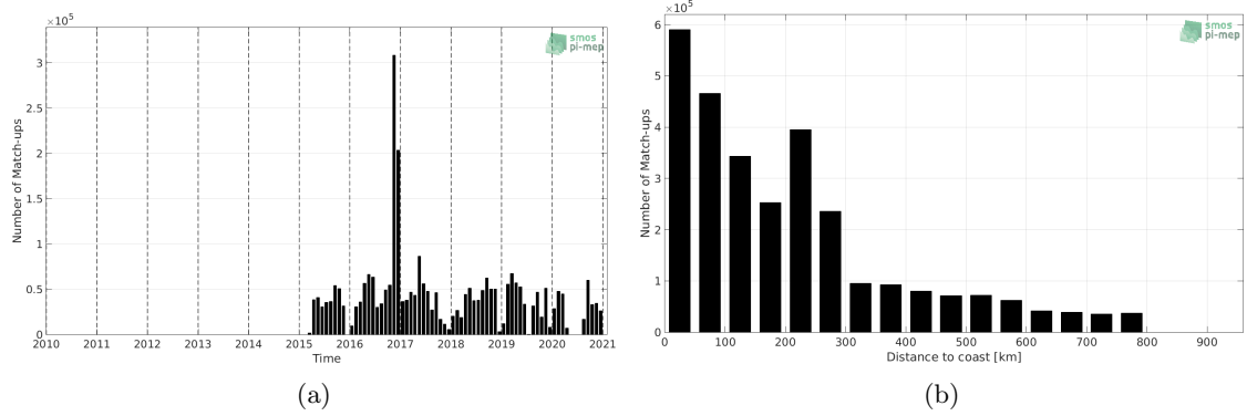
Figure 1: Number of match-ups between TSG (GOSUD-Research-vessel) and SMAP SSS L3 v4 - 8-Day running (RSS) SSS as a function of time (a) and as function of the distance to coast (b) over the SMOS coastal zone (<800km) 60N-60S Pi-MEP region and for the full satellite product period.
