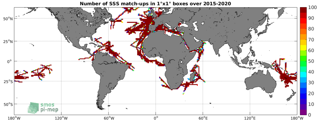
Figure 4: Number of SSS match-ups between TSG (GOSUD-Research-vessel) SSS and the SMAP SSS L3 v4 - 8-Day running (RSS) SSS product for the SMOS coastal zone (<800km) 60N-60S Pi-MEP region over 1^\circ \times 1^\circ boxes and for the full satellite product period.
