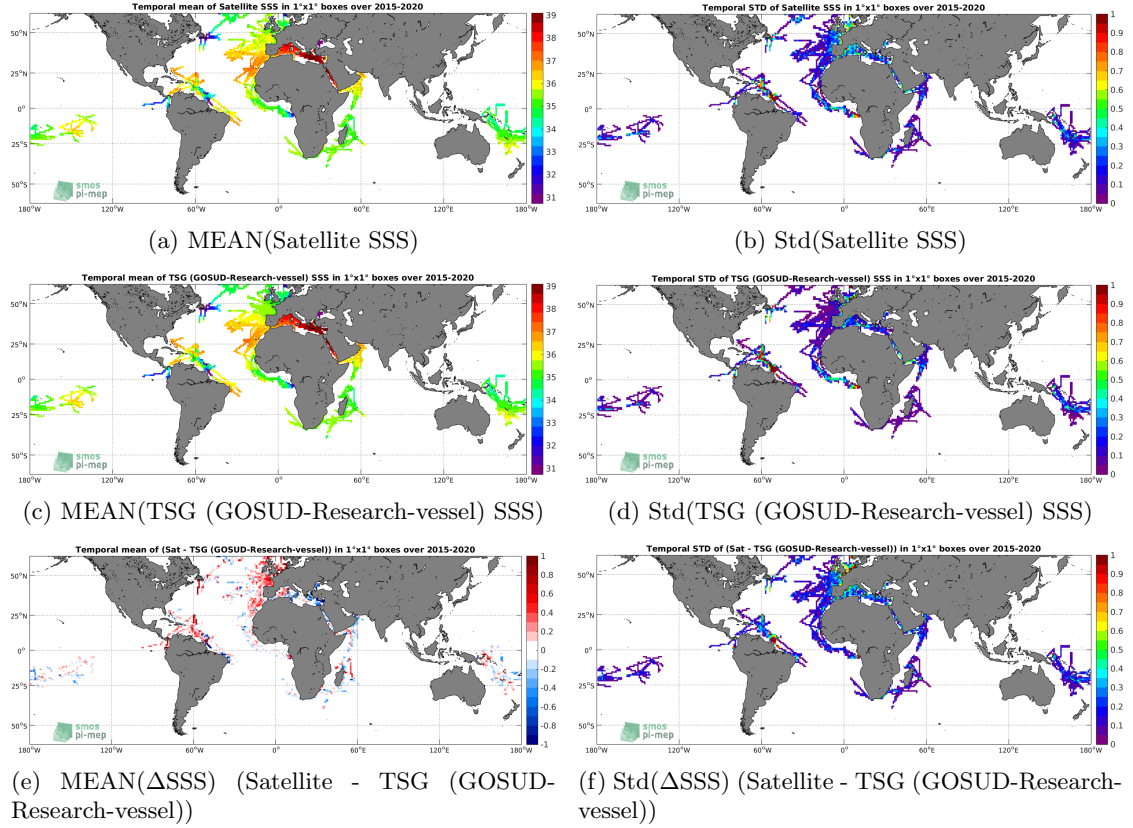
Figure 6: Temporal mean (left) and Std (right) of SSS from SMAP SSS L3 v4 - 8-Day running (RSS) (top), TSG (GOSUD-Research-vessel) (middle), and of \Delta SSS (Satellite - TSG (GOSUD-Research-vessel)). Only match-up pairs are used to generate these maps.
