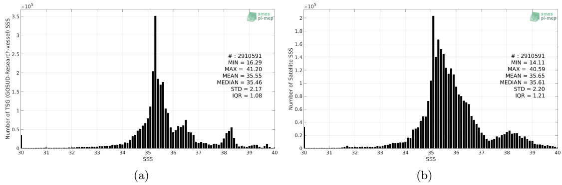
Figure 2: Histograms of SSS from TSG (GOSUD-Research-vessel) (a) and SMAP SSS L3 v4 - 8-Day running (RSS) (b) considering all match-up pairs per bins of 0.1 over the SMOS coastal zone (<800km) 60N-60S Pi-MEP region and for the full satellite product period.
