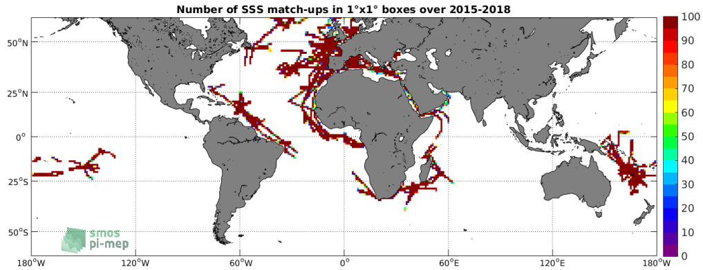
Figure 4: Number of SSS match-ups between TSG-GOSUD-Research-vessel SSS and the SMAP-L3-RSS-V4-8DAY-RUNNING SSS product for the SMOS coastal zone ( \pm 800\text{km} ) 60N-60S Pi-MEP region over 1^\circ \times 1^\circ boxes and for the full satellite product period.
