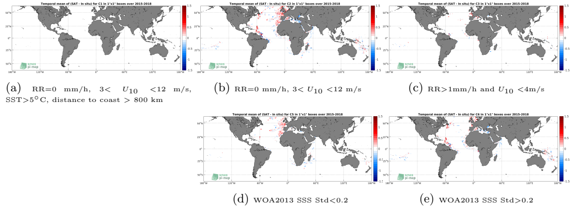
Figure 12: Temporal mean gridded over spatial boxes of size 1^\circ \times 1^\circ of \Delta SSS (SMAP-L3-RSS-V4-8DAY-RUNNING - TSG-GOSUD-Research-vessel) for 5 different subdatasets corresponding to: RR=0 mm/h, 3 < U_{10} < 12 m/s, SST > 5^\circ C , distance to coast > 800 km (a), RR=0 mm/h, 3 < U_{10} < 12 m/s (b), RR > 1 mm/h and U_{10} < 4 m/s (c), WOA2013 SSS Std < 0.2 (d), WOA2013 SSS Std > 0.2 (e).
