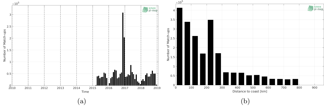
Figure 1: Number of match-ups between TSG-GOSUD-Research-vessel and SMAP-L3-RSS-V4-8DAY-RUNNING SSS as a function of time (a) and as function of the distance to coast (b) over the SMOS coastal zone ( \leq 800 km) 60N-60S Pi-MEP region and for the full satellite product period.
