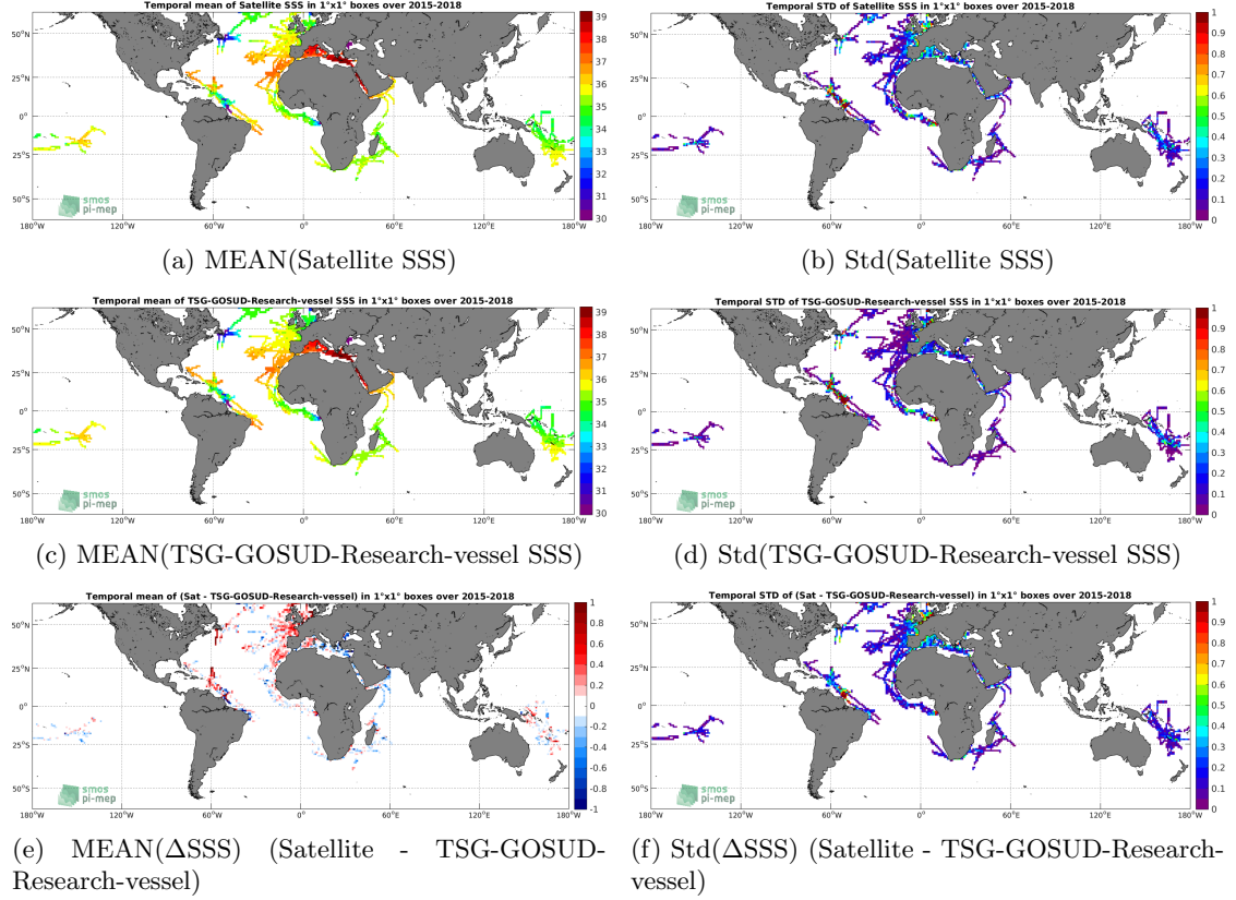
Figure 6: Temporal mean (left) and Std (right) of SSS from SMAP-L3-RSS-V4-8DAY-RUNNING (top), TSG-GOSUD-Research-vessel (middle), and of \Delta SSS (Satellite - TSG-GOSUD-Research-vessel). Only match-up pairs are used to generate these maps.
