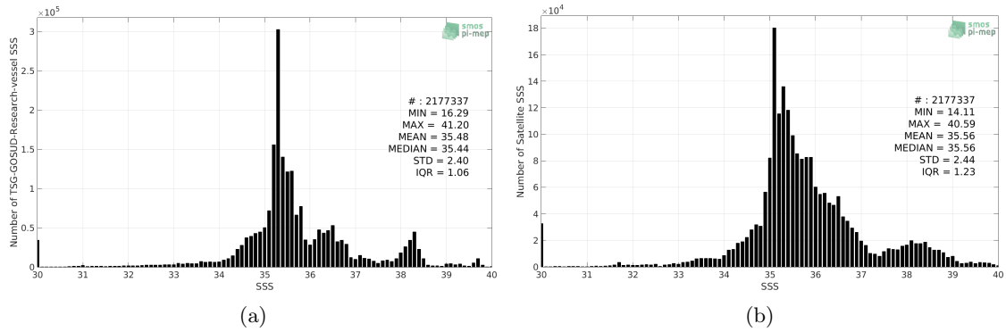
Figure 2: Histograms of SSS from TSG-GOSUD-Research-vessel (a) and SMAP-L3-RSS-V4-8DAY-RUNNING (b) considering all match-up pairs per bins of 0.1 over the SMOS coastal zone ( \leq 800 km) 60N-60S Pi-MEP region and for the full satellite product period.
