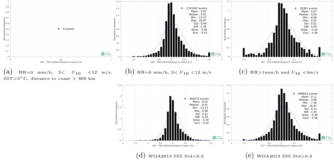
Figure 13: Normalized histogram of \Delta SSS (SMAP-L3-RSS-V4-8DAY-RUNNING - TSG-GOSUD-Research-vessel) for 5 different subdatasets corresponding to: RR=0 mm/h, 3 < U_{10} < 12 m/s, SST > 5^\circ C , distance to coast > 800 km (a), RR=0 mm/h, 3 < U_{10} < 12 m/s (b), RR > 1 mm/h and U_{10} < 4 m/s (c), WOA2013 SSS Std < 0.2 (d), WOA2013 SSS Std > 0.2 (e).
