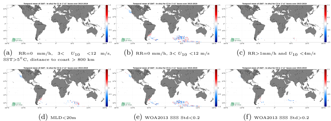
Figure 12: Temporal mean gridded over spatial boxes of size 1^\circ \times 1^\circ of \Delta SSS (SMAP SSS L3 v4 - 8-Day running (RSS) - Marine mammals) for 6 different subdatasets corresponding to:RR=0 mm/h, 3 < U_{10} < 12 m/s, SST >5^\circ C, distance to coast > 800 km (a), RR=0 mm/h, 3 < U_{10} < 12 m/s (b), RR >1 mm/h and U_{10} < 4 m/s (c),MLD <20 m (d),WOA2013 SSS Std <0.2 (e),WOA2013 SSS Std >0.2 (f).
