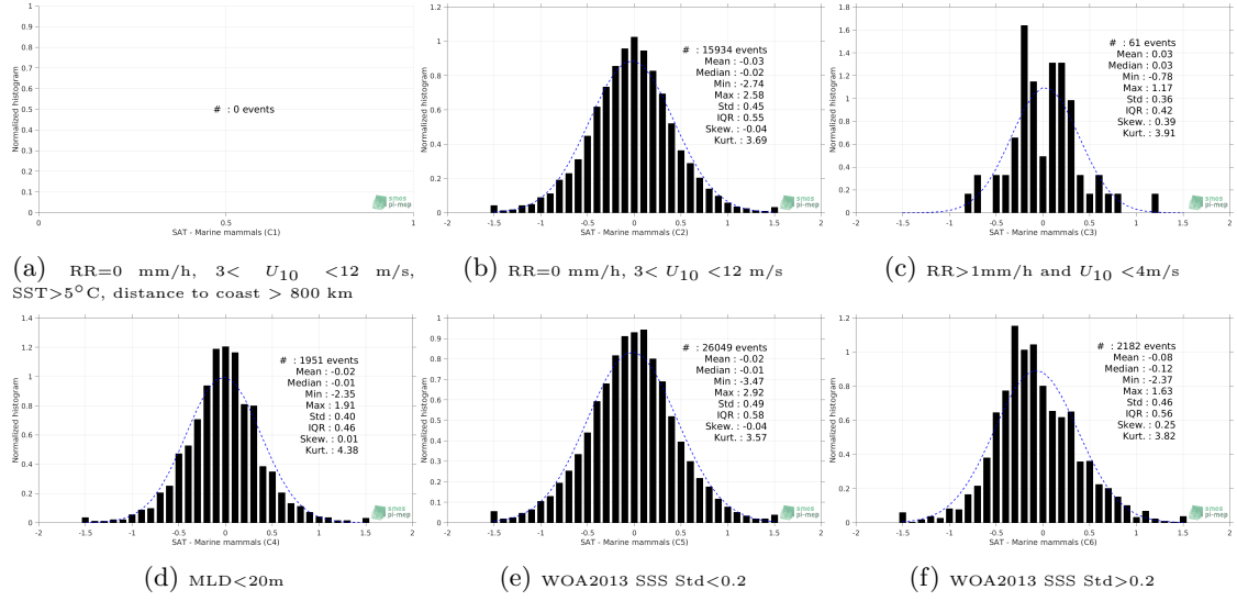
Figure 13: Normalized histogram of \Delta SSS (SMAP SSS L3 v4 - 8-Day running (RSS) - Marine mammals) for 6 different subdatasets corresponding to: RR=0 mm/h, 3 < U_{10} < 12 m/s, SST>5°C, distance to coast > 800 km (a), RR=0 mm/h, 3 < U_{10} < 12 m/s (b), RR>1mm/h and U_{10} < 4 m/s (c), MLD<20m (d), WOA2013 SSS Std<0.2 (e), WOA2013 SSS Std>0.2 (f).
