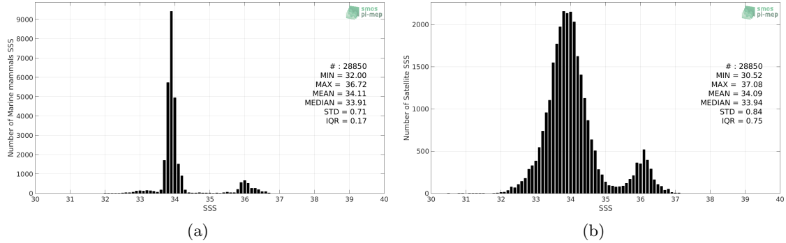
Figure 2: Histograms of SSS from Marine mammals (a) and SMAP SSS L3 v4 - 8-Day running (RSS) (b) considering all match-up pairs per bins of 0.1 over the SMOS coastal zone (<800km) 60N-60S Pi-MEP region and for the full satellite product period.
