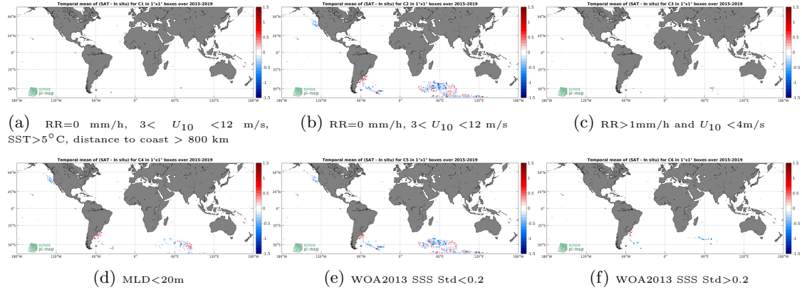
Figure 12: Temporal mean gridded over spatial boxes of size 1^\circ \times 1^\circ of \Delta SSS (SMAP SSS L3 v4 - 8-Day running (RSS) - Marine mammals) for 6 different subdatasets corresponding to: RR=0 mm/h, 3 < U_{10} < 12 m/s, SST > 5^\circ C , distance to coast > 800 km (a), RR=0 mm/h, 3 < U_{10} < 12 m/s (b), RR > 1 mm/h and U_{10} < 4 m/s (c), MLD < 20 m (d), WOA2013 SSS Std < 0.2 (e), WOA2013 SSS Std > 0.2 (f).
