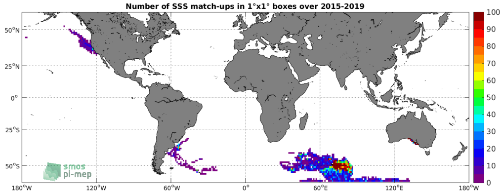
Figure 4: Number of SSS match-ups between Marine mammals SSS and the SMAP SSS L3 v4 - 8-Day running (RSS) SSS product for the SMOS coastal zone (<800km) 60N-60S Pi-MEP region over 1^\circ \times 1^\circ boxes and for the full satellite product period.
