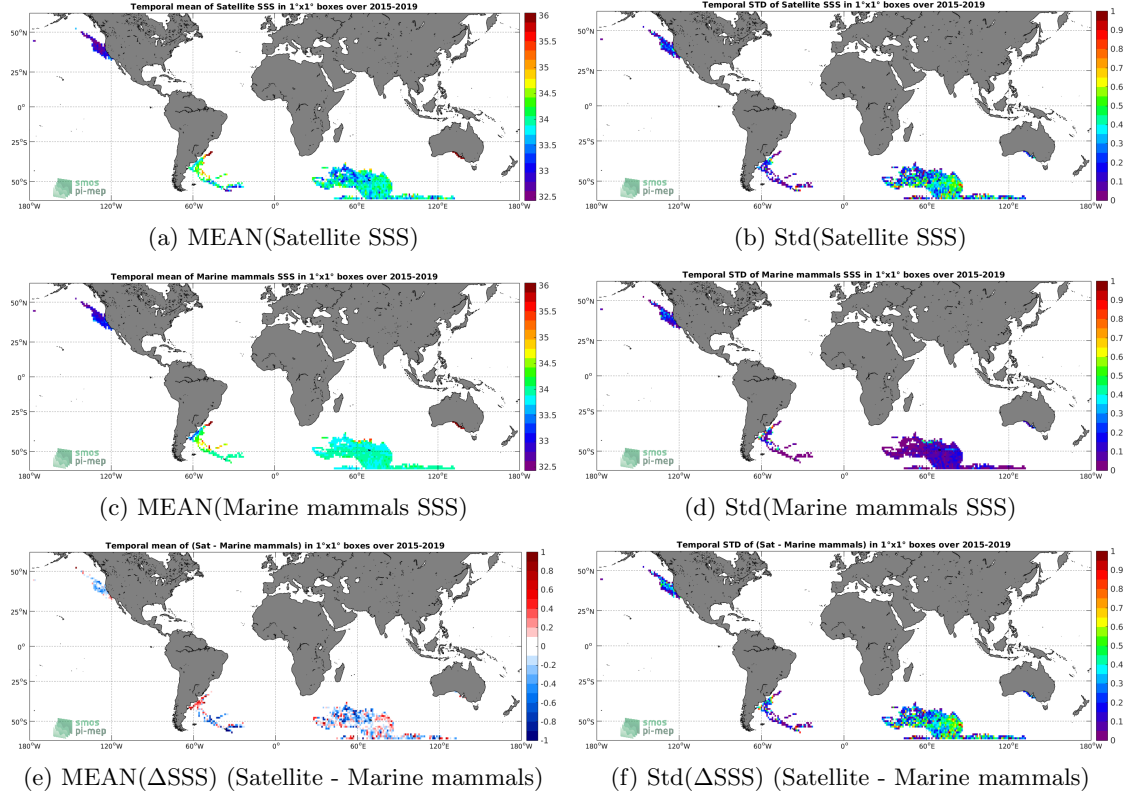
Figure 6: Temporal mean (left) and Std (right) of SSS from SMAP SSS L3 v4 - 8-Day running (RSS) (top), Marine mammals (middle), and of \Delta SSS (Satellite - Marine mammals). Only match-up pairs are used to generate these maps.
