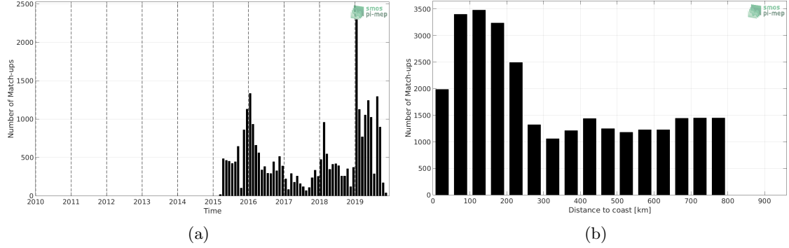
Figure 1: Number of match-ups between Marine mammals and SMAP SSS L3 v4 - 8-Day running (RSS) SSS as a function of time (a) and as function of the distance to coast (b) over the SMOS coastal zone (<800km) 60N-60S Pi-MEP region and for the full satellite product period.
