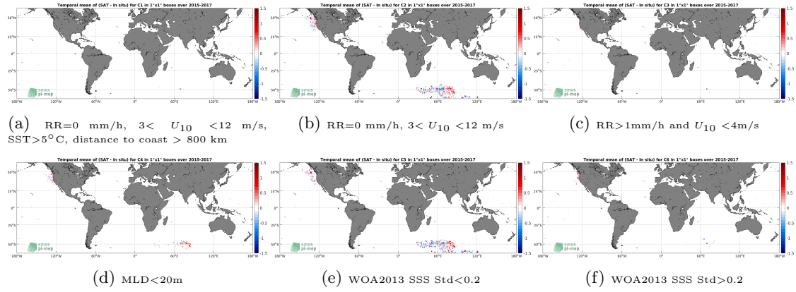
Figure 12: Temporal mean gridded over spatial boxes of size 1^\circ \times 1^\circ of \Delta SSS (SMAP SSS L3 v4 - 8-Day running (RSS) - Sea mammals) for 6 different subdatasets corresponding to: RR=0 mm/h, 3 < U_{10} < 12 m/s, SST > 5^\circ C , distance to coast > 800 km (a), RR=0 mm/h, 3 < U_{10} < 12 m/s (b), RR > 1 mm/h and U_{10} < 4 m/s (c), MLD < 20 m (d), WOA2013 SSS Std < 0.2 (e), WOA2013 SSS Std > 0.2 (f).
