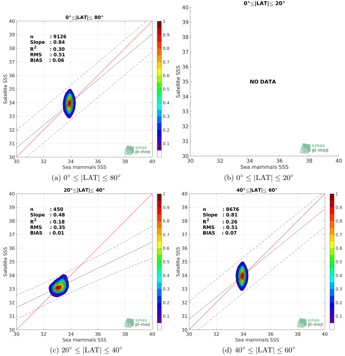
Figure 9: Contour maps of the concentration of SMAP SSS L3 v4 - 8-Day running (RSS) SSS (y-axis) versus Sea mammals SSS (x-axis) at match-up pairs for different latitude bands. For each plot, the red line shows x=y . The black thin and dashed lines indicate a linear fit through the data cloud and the \pm 95\% confidence levels, respectively. The number match-up pairs n , the slope and R^2 coefficient of the linear fit, the root mean square (RMS) and the mean bias between satellite and in situ data are indicated for each latitude band in each plots.
