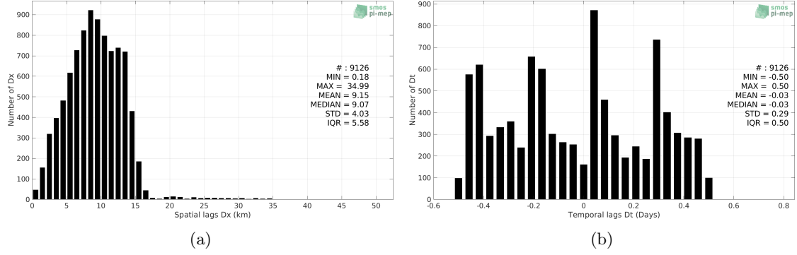
Figure 5: Histograms of the spatial (a) and temporal (b) lags between the location/time of the Sea mammals measurement and the date of the corresponding SMAP SSS L3 v4 - 8-Day running (RSS) SSS pixel.
