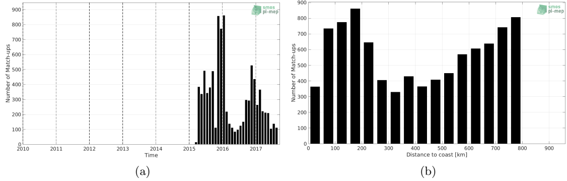
Figure 1: Number of match-ups between Sea mammals and SMAP SSS L3 v4 - 8-Day running (RSS) SSS as a function of time (a) and as function of the distance to coast (b) over the SMOS coastal zone (<800km) 60N-60S Pi-MEP region and for the full satellite product period.
