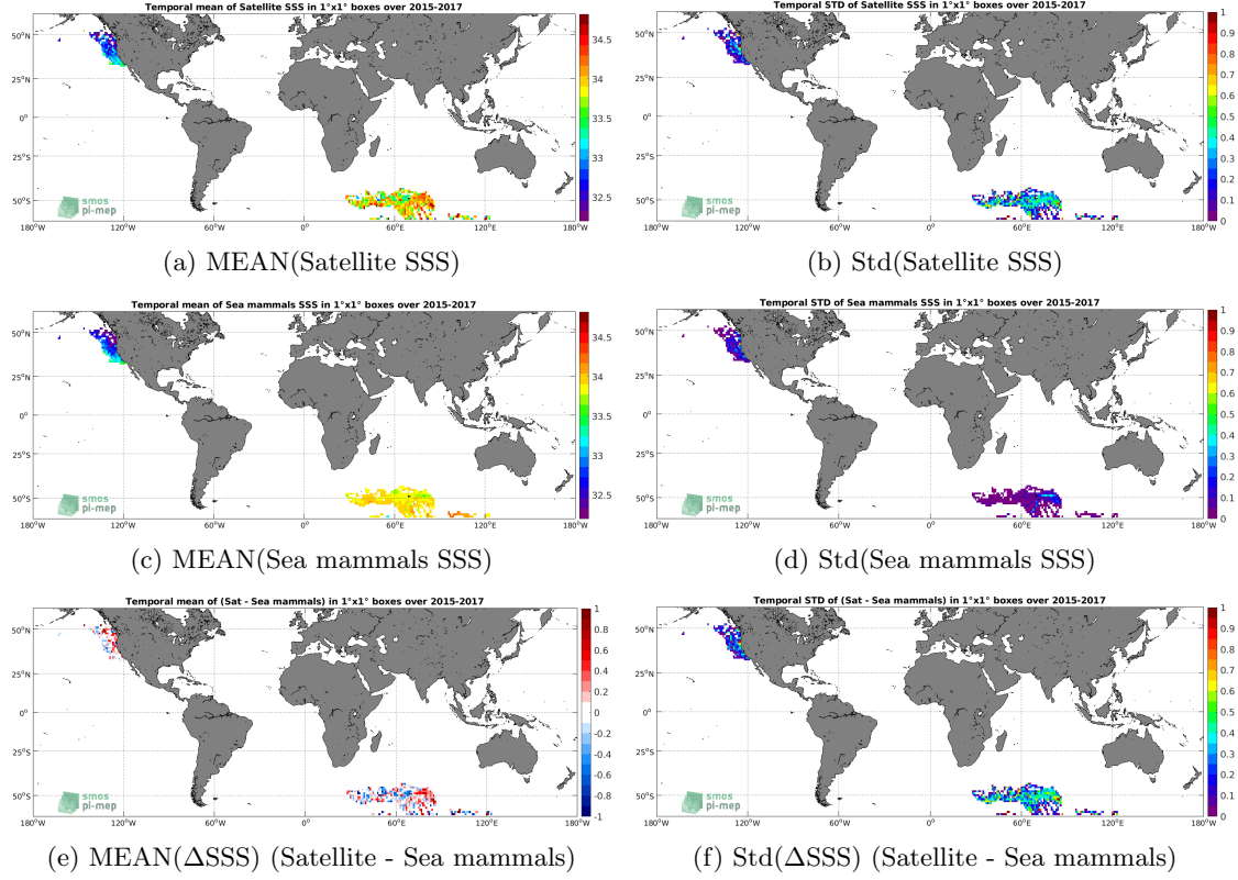
Figure 6: Temporal mean (left) and Std (right) of SSS from SMAP SSS L3 v4 - 8-Day running (RSS) (top), Sea mammals (middle), and of \Delta SSS (Satellite - Sea mammals). Only match-up pairs are used to generate these maps.
