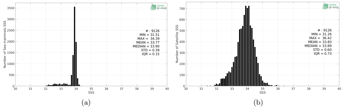
Figure 2: Histograms of SSS from Sea mammals (a) and SMAP SSS L3 v4 - 8-Day running (RSS) (b) considering all match-up pairs per bins of 0.1 over the SMOS coastal zone (<800km) 60N-60S Pi-MEP region and for the full satellite product period.
