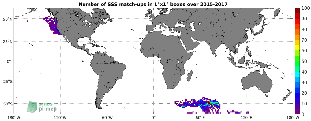
Figure 4: Number of SSS match-ups between Sea mammals SSS and the SMAP SSS L3 v4 - 8-Day running (RSS) SSS product for the SMOS coastal zone (<800km) 60N-60S Pi-MEP region over 1^\circ \times 1^\circ boxes and for the full satellite product period.
