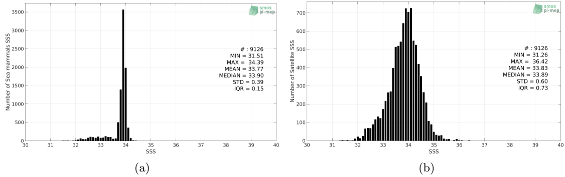
Figure 2: Histograms of SSS from Sea mammals (a) and SMAP-L3-RSS-V4-8DAY-RUNNING (b) considering all match-up pairs per bins of 0.1 over the SMOS coastal zone (<800km) 60N-60S Pi-MEP region and for the full satellite product period.
