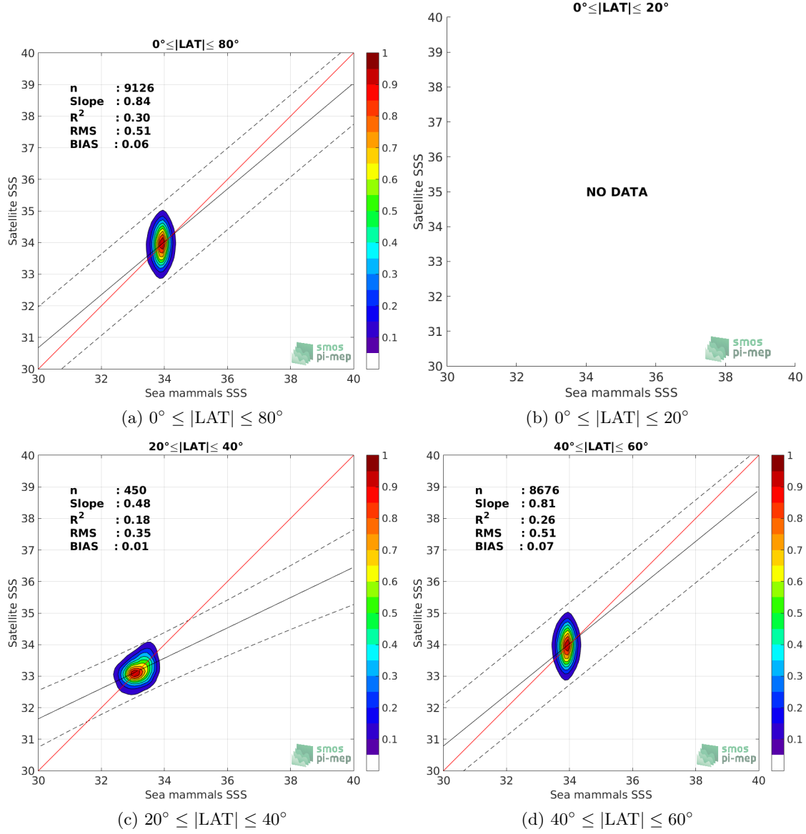
Figure 9: Contour maps of the concentration of SMAP-L3-RSS-V4-8DAY-RUNNING SSS (y-axis) versus Sea mammals SSS (x-axis) at match-up pairs for different latitude bands. For each plot, the red line shows x=y . The black thin and dashed lines indicate a linear fit through the data cloud and the \pm 95\% confidence levels, respectively. The number match-up pairs n , the slope and R^2 coefficient of the linear fit, the root mean square (RMS) and the mean bias between satellite and in situ data are indicated for each latitude band in each plots.
