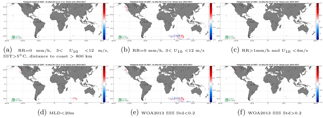
Figure 12: Temporal mean gridded over spatial boxes of size 1^\circ \times 1^\circ of \Delta SSS (SMAP-L3-RSS-V4-8DAY-RUNNING - Sea mammals) for 6 different subdatasets corresponding to: RR=0 mm/h, 3 < U_{10} < 12 m/s, SST > 5^\circ C , distance to coast > 800 km (a), RR=0 mm/h, 3 < U_{10} < 12 m/s (b), RR > 1 mm/h and U_{10} < 4 m/s (c), MLD < 20 m (d), WOA2013 SSS Std < 0.2 (e), WOA2013 SSS Std > 0.2 (f).
