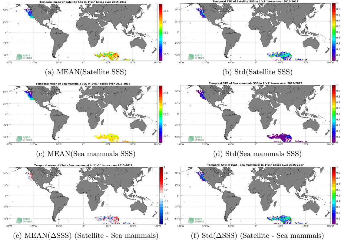
Figure 6: Temporal mean (left) and Std (right) of SSS from SMAP-L3-RSS-V4-8DAY-RUNNING (top), Sea mammals (middle), and of \Delta SSS (Satellite - Sea mammals). Only match-up pairs are used to generate these maps.
