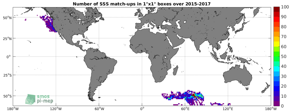
Figure 4: Number of SSS match-ups between Sea mammals SSS and the SMAP-L3-RSS-V4-8DAY-RUNNING SSS product for the SMOS coastal zone ( \pm 800\text{km} ) 60N-60S Pi-MEP region over 1^\circ \times 1^\circ boxes and for the full satellite product period.
