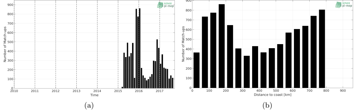
Figure 1: Number of match-ups between Sea mammals and SMAP-L3-RSS-V4-8DAY-RUNNING SSS as a function of time (a) and as function of the distance to coast (b) over the SMOS coastal zone ( \geq 800\text{km} ) 60N-60S Pi-MEP region and for the full satellite product period.
