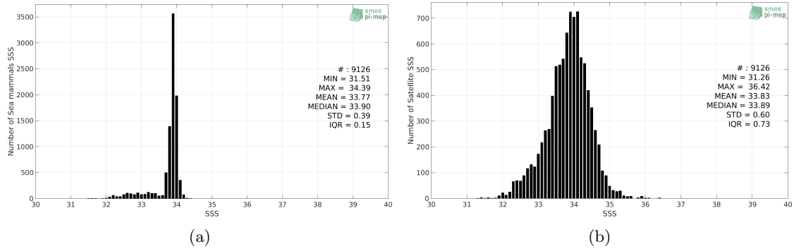
Figure 2: Histograms of SSS from Sea mammals (a) and SMAP-L3-RSS-V4-8DAY-RUNNING (b) considering all match-up pairs per bins of 0.1 over the SMOS coastal zone ( \geq 800\text{km} ) 60N-60S Pi-MEP region and for the full satellite product period.
