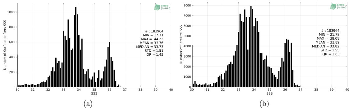
Figure 2: Histograms of SSS from Surface drifters (a) and SMAP SSS L3 v4 - 8-Day running (RSS) (b) considering all match-up pairs per bins of 0.1 over the SMOS coastal zone (<800km) 60N-60S Pi-MEP region and for the full satellite product period.
