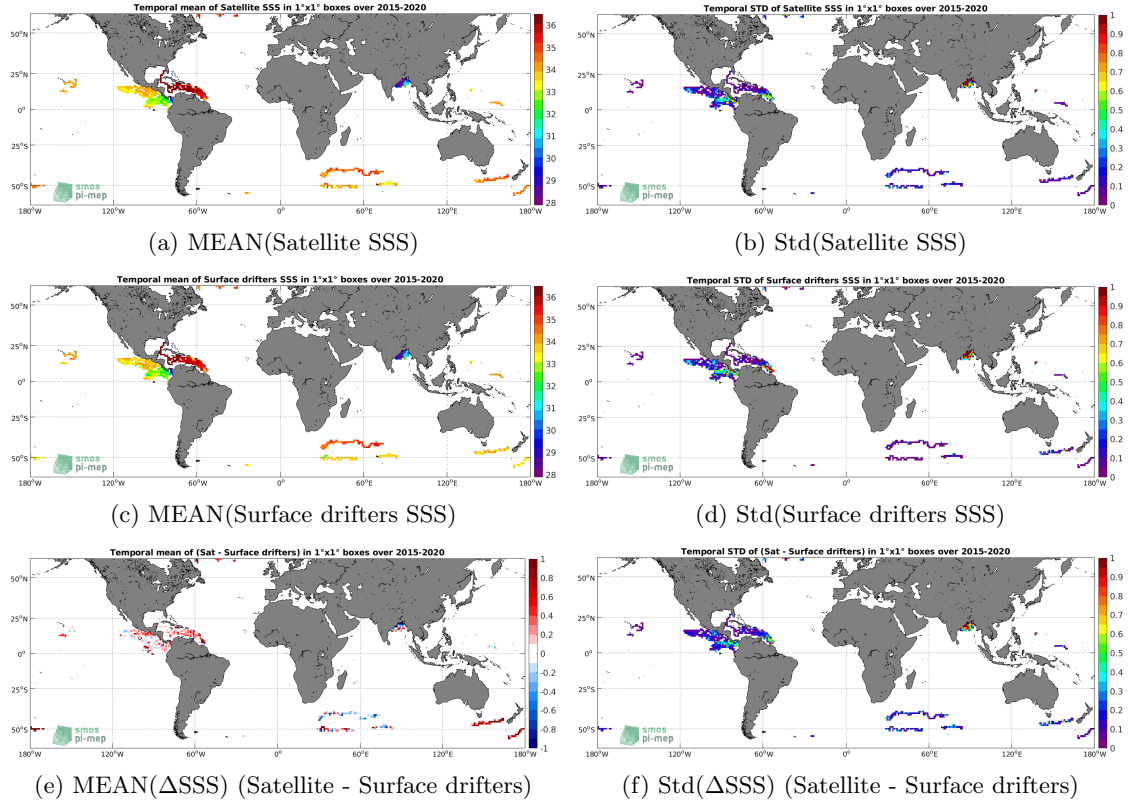
Figure 5: Temporal mean (left) and Std (right) of SSS from SMAP SSS L3 v4 - 8-Day running (RSS) (top), Surface drifters (middle), and of \Delta SSS (Satellite - Surface drifters). Only match-up pairs are used to generate these maps.
