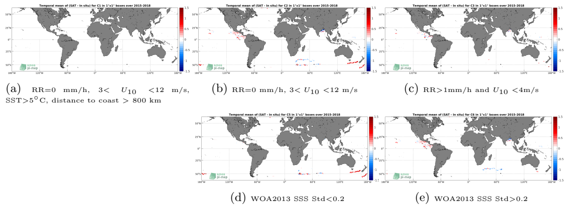
Figure 11: Temporal mean gridded over spatial boxes of size 1^\circ \times 1^\circ of \Delta\text{SSS} (SMAP SSS L3 v4 - 8-Day running (RSS) - Surface drifters) for 5 different subdatasets corresponding to: RR=0 mm/h, 3 < U_{10} < 12 m/s, SST > 5^\circ\text{C} , distance to coast > 800 km (a), RR=0 mm/h, 3 < U_{10} < 12 m/s (b), RR > 1 mm/h and U_{10} < 4 m/s (c), WOA2013 SSS Std < 0.2 (d), WOA2013 SSS Std > 0.2 (e).
