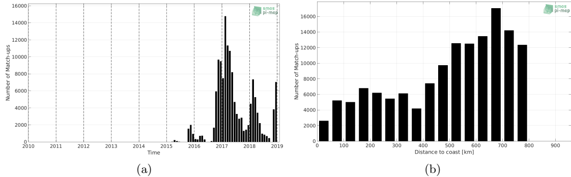
Figure 1: Number of match-ups between Surface drifters and SMAP-L3-RSS-V4-8DAY-RUNNING SSS as a function of time (a) and as function of the distance to coast (b) over the SMOS coastal zone (<800km) 60N-60S Pi-MEP region and for the full satellite product period.
