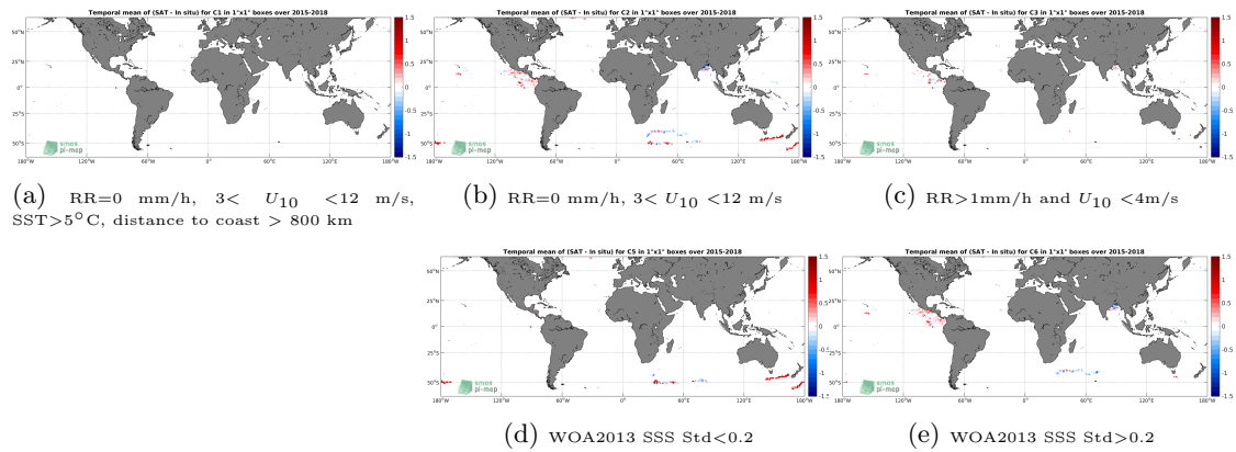
Figure 11: Temporal mean gridded over spatial boxes of size 1^\circ \times 1^\circ of \Delta SSS (SMAP-L3-RSS-V4-8DAY-RUNNING - Surface drifters) for 5 different subdatasets corresponding to:RR=0 mm/h, 3 < U_{10} < 12 m/s, SST >5^\circ\text{C} , distance to coast > 800 km (a), RR=0 mm/h, 3 < U_{10} < 12 m/s (b), RR >1 mm/h and U_{10} < 4 m/s (c), WOA2013 SSS Std <0.2 (d), WOA2013 SSS Std >0.2 (e).
