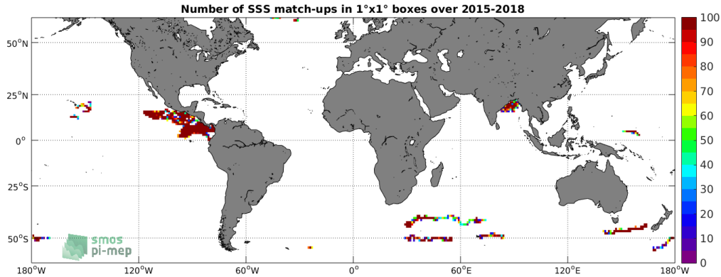
Figure 3: Number of SSS match-ups between Surface drifters SSS and the SMAP-L3-RSS-V4-8DAY-RUNNING SSS product for the SMOS coastal zone (<800km) 60N-60S Pi-MEP region over 1^\circ \times 1^\circ boxes and for the full satellite product period.
