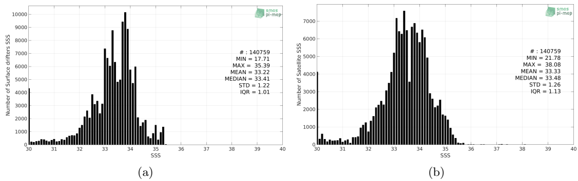
Figure 2: Histograms of SSS from Surface drifters (a) and SMAP-L3-RSS-V4-8DAY-RUNNING (b) considering all match-up pairs per bins of 0.1 over the SMOS coastal zone (<800km) 60N-60S Pi-MEP region and for the full satellite product period.
