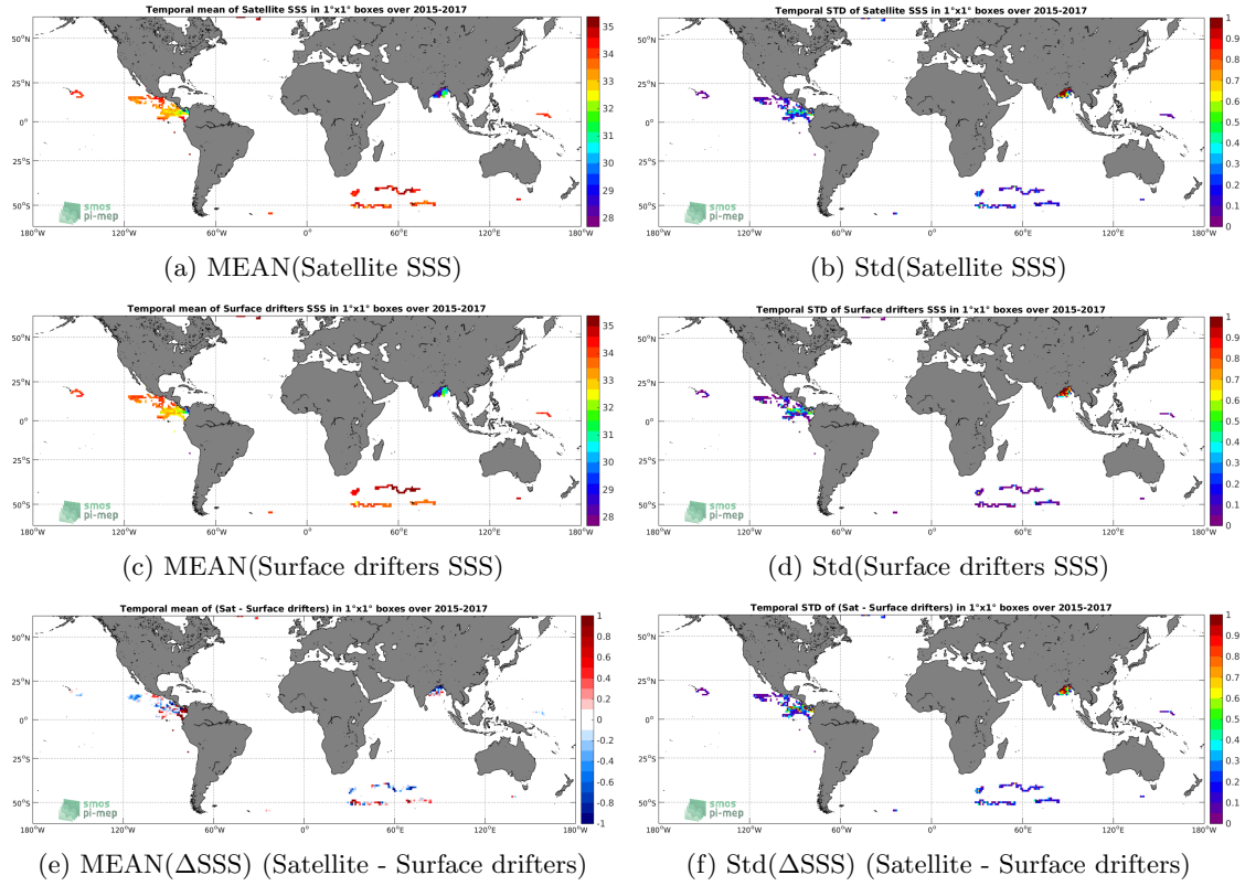
Figure 5: Temporal mean (left) and Std (right) of SSS from SMAP-L3-RSS-V4-8DAY-RUNNING (top), Surface drifters (middle), and of \Delta SSS (Satellite - Surface drifters). Only match-up pairs are used to generate these maps.
