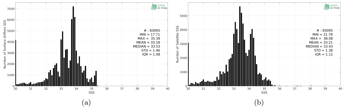
Figure 2: Histograms of SSS from Surface drifters (a) and SMAP-L3-RSS-V4-8DAY-RUNNING (b) considering all match-up pairs per bins of 0.1 over the SMOS coastal zone ( \pm 800\text{km} ) 60N-60S Pi-MEP region and for the full satellite product period.
