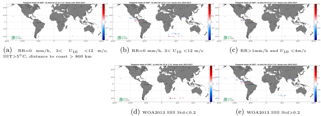
Figure 11: Temporal mean gridded over spatial boxes of size 1^\circ \times 1^\circ of \Delta SSS (SMAP-L3-RSS-V4-8DAY-RUNNING - Surface drifters) for 5 different subdatasets corresponding to: RR=0 mm/h, 3 < U_{10} < 12 m/s, SST > 5^\circ C , distance to coast > 800 km (a), RR=0 mm/h, 3 < U_{10} < 12 m/s (b), RR > 1 mm/h and U_{10} < 4 m/s (c), WOA2013 SSS Std < 0.2 (d), WOA2013 SSS Std > 0.2 (e).
