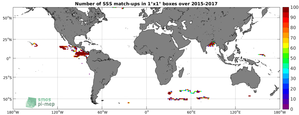
Figure 3: Number of SSS match-ups between Surface drifters SSS and the SMAP-L3-RSS-V4-8DAY-RUNNING SSS product for the SMOS coastal zone ( \pm 800\text{km} ) 60N-60S Pi-MEP region over 1^\circ \times 1^\circ boxes and for the full satellite product period.
