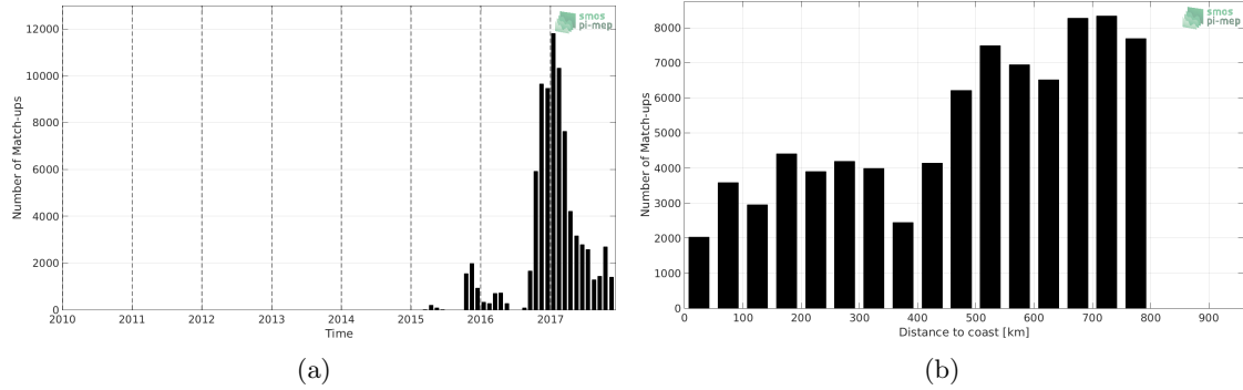
Figure 1: Number of match-ups between Surface drifters and SMAP-L3-RSS-V4-8DAY-RUNNING SSS as a function of time (a) and as function of the distance to coast (b) over the SMOS coastal zone ( \pm 800\text{km} ) 60N-60S Pi-MEP region and for the full satellite product period.
