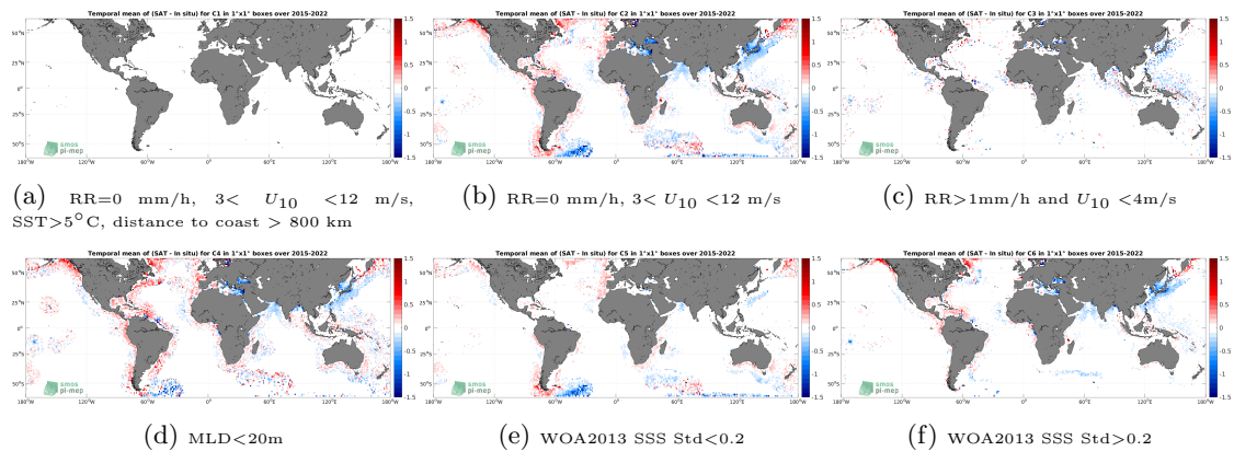
Figure 12: Temporal mean gridded over spatial boxes of size 1^\circ \times 1^\circ of \Delta SSS (SMAP SSS L3 v4 - 8-Day running (RSS) - Argo) for 6 different subdatasets corresponding to:RR=0 mm/h, 3 < U_{10} < 12 m/s, SST >5^\circ C, distance to coast > 800 km (a), RR=0 mm/h, 3 < U_{10} < 12 m/s (b), RR >1 mm/h and U_{10} < 4 m/s (c),MLD <20 m (d),WOA2013 SSS Std <0.2 (e),WOA2013 SSS Std >0.2 (f).
