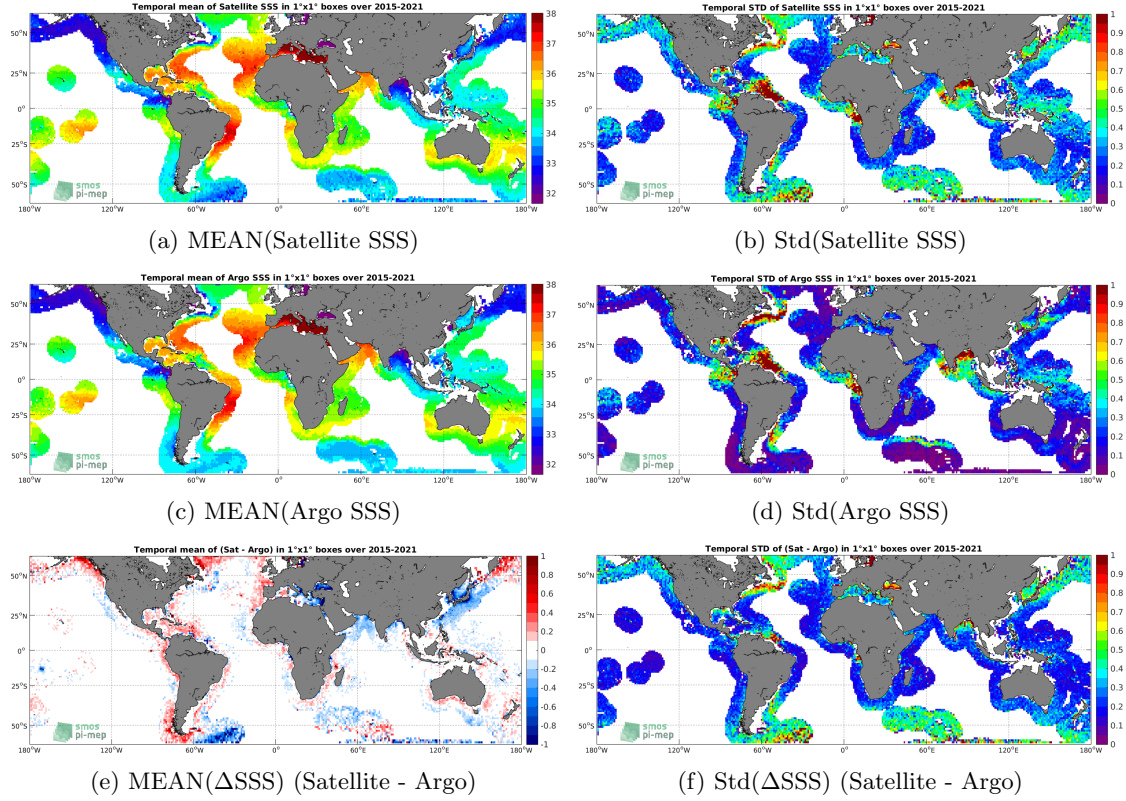
Figure 6: Temporal mean (left) and Std (right) of SSS from SMAP SSS L3 v4 - 8-Day running (RSS) (top), Argo (middle), and of \Delta SSS (Satellite - Argo). Only match-up pairs are used to generate these maps.
