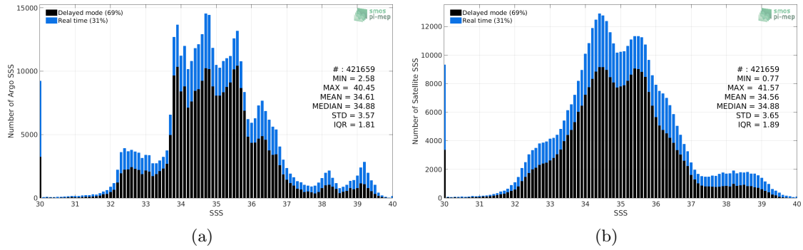
Figure 2: Histograms of SSS from Argo (a) and SMAP SSS L3 v4 - 8-Day running (RSS) (b) considering all match-up pairs per bins of 0.1 over the SMOS coastal zone (<800km) 60N-60S Pi-MEP region and for the full satellite product period.
