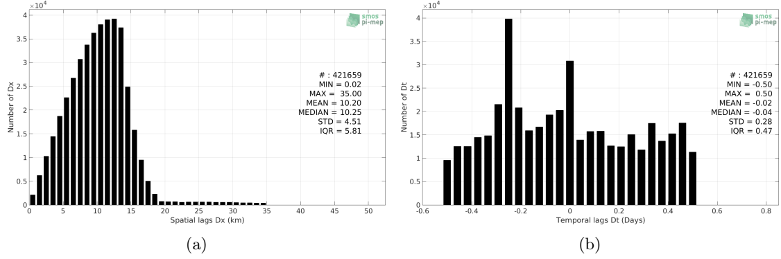
Figure 5: Histograms of the spatial (a) and temporal (b) lags between the location/time of the Argo measurement and the date of the corresponding SMAP SSS L3 v4 - 8-Day running (RSS) SSS pixel.
