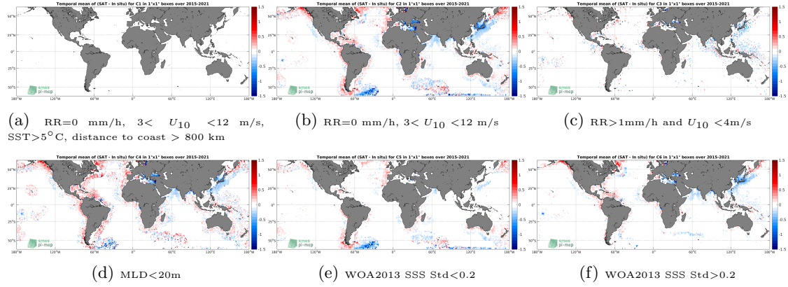
Figure 12: Temporal mean gridded over spatial boxes of size 1^\circ \times 1^\circ of \Delta SSS (SMAP SSS L3 v4 - 8-Day running (RSS) - Argo) for 6 different subdatasets corresponding to: RR=0 mm/h, 3 < U_{10} < 12 m/s, SST > 5^\circ\text{C} , distance to coast > 800 km (a), RR=0 mm/h, 3 < U_{10} < 12 m/s (b), RR > 1 mm/h and U_{10} < 4 m/s (c), MLD < 20 m (d), WOA2013 SSS Std < 0.2 (e), WOA2013 SSS Std > 0.2 (f).
