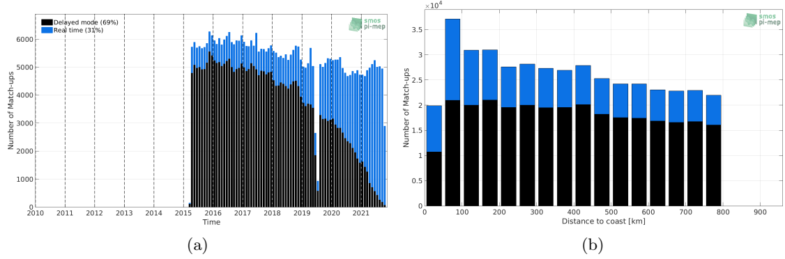
Figure 1: Number of match-ups between Argo and SMAP SSS L3 v4 - 8-Day running (RSS) SSS as a function of time (a) and as function of the distance to coast (b) over the SMOS coastal zone (<800km) 60N-60S Pi-MEP region and for the full satellite product period.
