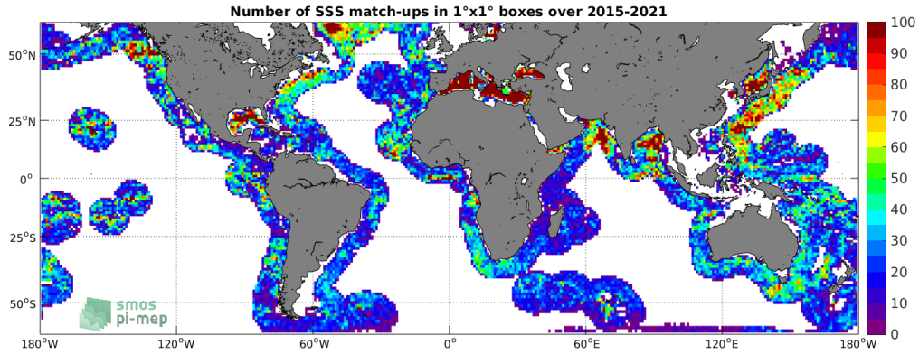
Figure 4: Number of SSS match-ups between Argo SSS and the SMAP SSS L3 v4 - 8-Day running (RSS) SSS product for the SMOS coastal zone (<800km) 60N-60S Pi-MEP region over 1^\circ \times 1^\circ boxes and for the full satellite product period.
