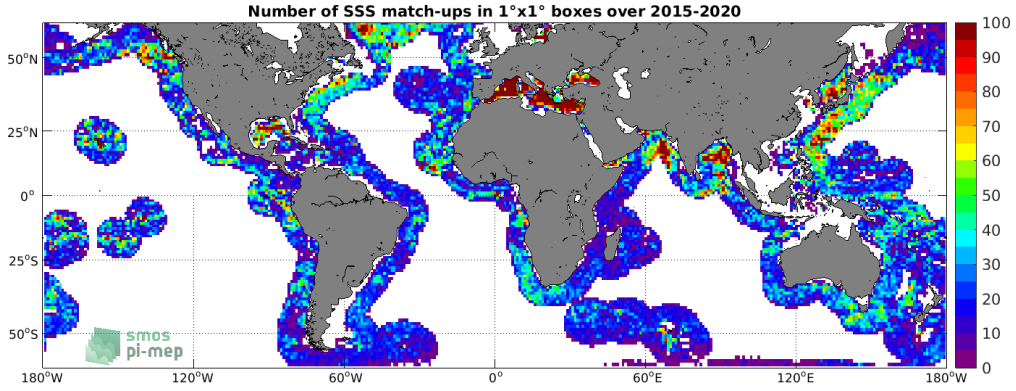
Figure 4: Number of SSS match-ups between Argo SSS and the SMAP SSS L3 v4 - 8-Day running (RSS) SSS product for the SMOS coastal zone (<800km) 60N-60S Pi-MEP region over 1°x1° boxes and for the full satellite product period.
