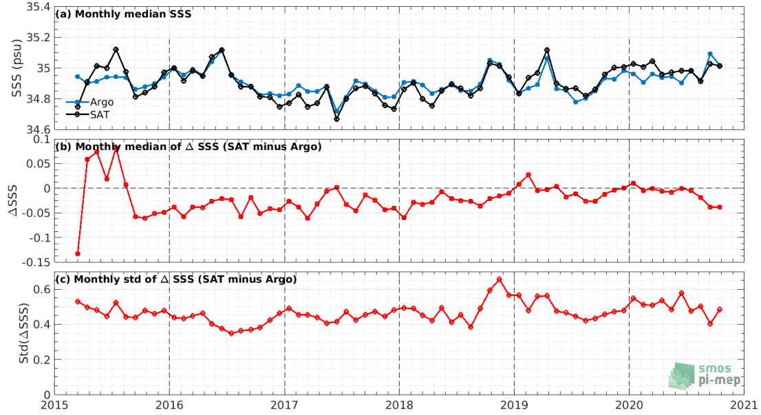
Figure 7: Time series of the monthly median SSS (top), median of \Delta\text{SSS} (Satellite - Argo) and Std of \Delta\text{SSS} (Satellite - Argo) over the SMOS coastal zone ( <800\text{km} ) 60\text{N} - 60\text{S} Pi-MEP region considering all match-ups collected by the Pi-MEP.
