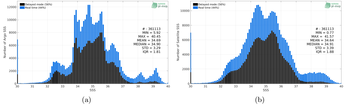
Figure 2: Histograms of SSS from Argo (a) and SMAP SSS L3 v4 - 8-Day running (RSS) (b) considering all match-up pairs per bins of 0.1 over the SMOS coastal zone (<800km) 60N-60S Pi-MEP region and for the full satellite product period.
